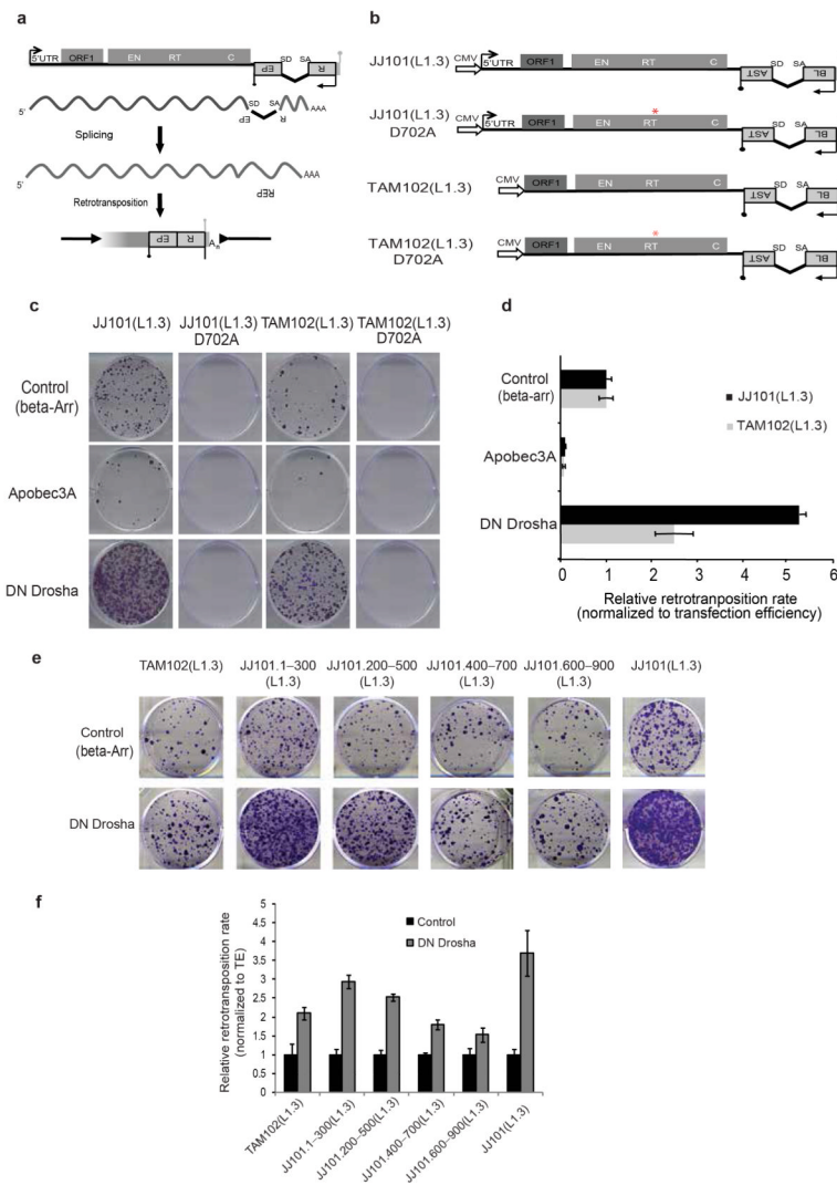
Figure 4. The Microprocessor negatively regulates L1 retrotransposition in vivo . (a) Cartoon depicting the LINE-1 based retrotransposition assay in cultured cells. The transcription start site at the L1 5' UTR (black arrow), the L1 open reading frames (ORF1 and ORF2; gray rectangles), and the L1 poly (A) site (grey lollipop) are indicated. The relative locations of the endonuclease (EN), reverse transcriptase (RT), and cysteine-rich (C) domains of ORF2 are also indicated. (b) Schematic representation of the JJ101(L1.3) vector containing a full-length human RC-L1 sequence tagged with a mblastI cassette (Blasticidin-resistance gene). The 5' UTR of L1.3 was removed to generate construct TAM102(L1.3). Alleles containing a missense mutation in the Reverse Transcriptase (RT) domain of L1-ORF2 (red asterisk, JJ101 (L1.3) D702A and TAM102 (L1.3) D702A) were used as an internal control. CMV denotes the presence of a Cytomegalovirus promoter. Black and grey lollipops represent polyadenylation signals. (c,e) Cell culture-based LINE-1 retrotransposition assay. (c) HeLa cells were co-transfected with JJ101(L1.3), TAM102(L1.3) and corresponding control vectors or the indicated engineered LINE-1 construct containing an individual fragment derived from the 5' UTR region plus the indicated expression plasmids (-arrestin (-arr), Apobec3A, or DN Drosha), as indicated on the left. Each image shows representative data from L1 retrotransposition assays conducted in triplicate. (d,f) Quantification of LINE-1
