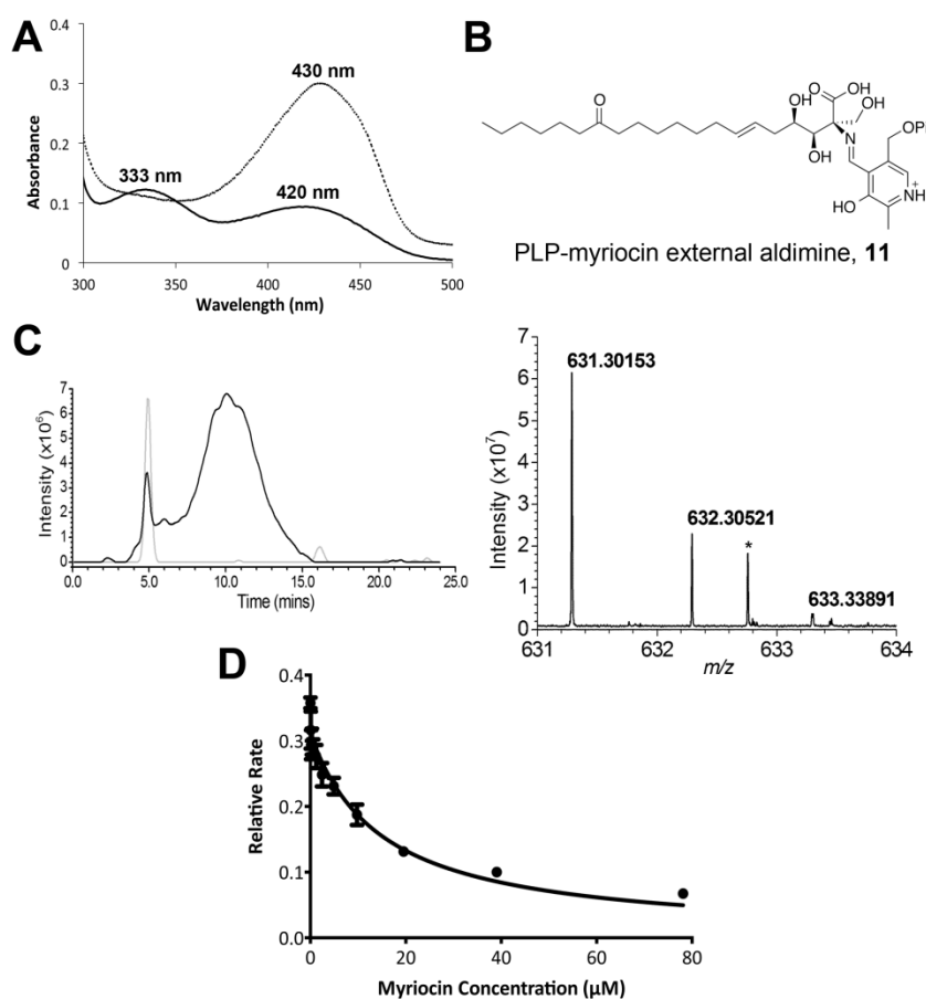
Figure 2. SPT inhibition occurs via formation of a PLP-myriocin aldimine. (A) UV-Vis spectrum of 40 \mu M SPT before (solid line) and after 200 \mu M myriocin addition (dotted line). (B) The proposed structure of the inhibitory complex - a PLP-myriocin aldimine, 11 . (C) Detection of the PLP-myriocin aldimine by LC-MS. Top , Extracted Ion Chromatogram at m/z 631. Bottom , high resolution mass spectrum of the PLP-myriocin
