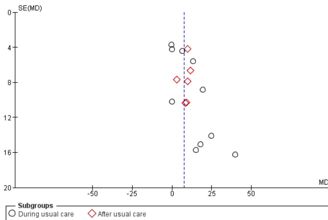
Figure 4. Funnel plot of comparison: I Cardiorespiratory training versus control - end of intervention, outcome: I.12 Mobility - maximal gait speed (m/min over 5 to 10 metres).
