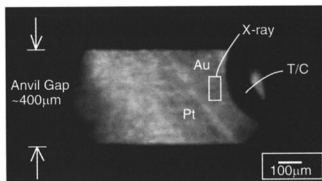
Figure 1. X-ray CCD image of the assembly at 21 GPa. The white square represents the area of 50 \times 100\text{-}\mu\text{m} , from which X-ray diffraction was collected. Both gold and platinum were closely loaded but separated by a thin layer of MgO to avoid metal alloying.
