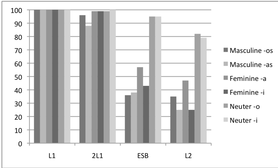
Figure 7. Greek: Average percentage of nouns with target determiner, separated by suffix
