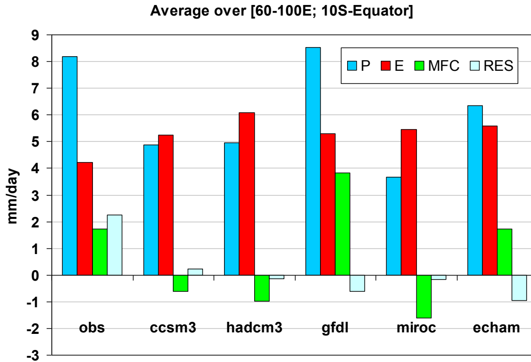
Figure 8: Seasonal (Jun-Sep) mean atmospheric water budget (in \text{mm day}^{-1} ; P = precipitation; E = evaporation; MFC = vertically-integrated moisture flux convergence) averaged over ( 60^{\circ} - 100^{\circ} E, 10^{\circ} S-Equator).
