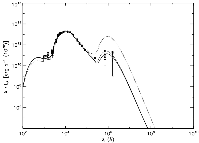
Figure 24. Comparison of theoretical elliptical model at 12 Gyr with an average SED taken from four elliptical galaxies of the SINGS sample. Solid line – full CPM08 model and dotted line – simple dust model. The thick line is for a scalelength of dust twice as large as that of the stellar component, while the thin line is for equal scalelengths.
