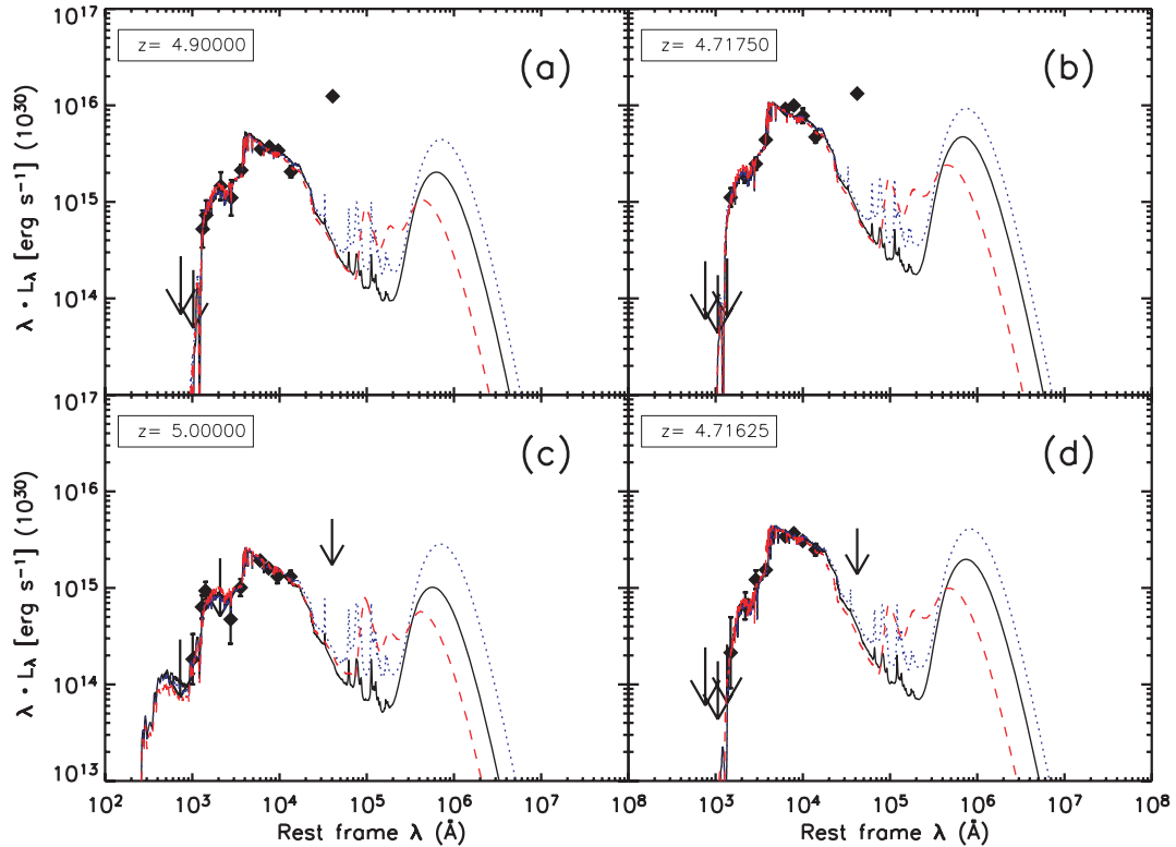
Figure 22. Comparison of the 10^{12} M_{\odot} theoretical elliptical model with the SED of balmer break galaxies. (a) BBG 2910, (b) BBG 3348, (c) BBG 3361, (d) BBG 4071. Black solid line – full CPM08 model. Blue dotted line – simple dust model. Red dashed line – full CPM08 model with dust consistent with the z \sim 6 QSO. The rest-frame wavelength is correct for the redshift calculated for the full CPM08 model, the value given in the top-left corner of the panel. In all cases, the redshift values were the same for the two other models; except for BBG 4071, where a redshift of 4.348 75 was calculated for the simple dust model, the abscissa values for the curve were appropriately rescaled. The redshift values calculated by Wiklind et al. (2008) are z = 4.9 for BBG 2910, z = 5.1 for BBG 3348, z = 5.0 for BBG 3361 and z = 5.0 for BBG 4071.
