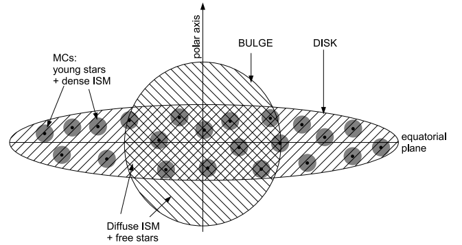
Figure 4. Sketch of geometry of stars and dust in the GRASIL model for the case of a galaxy with both a disc and a bulge.
