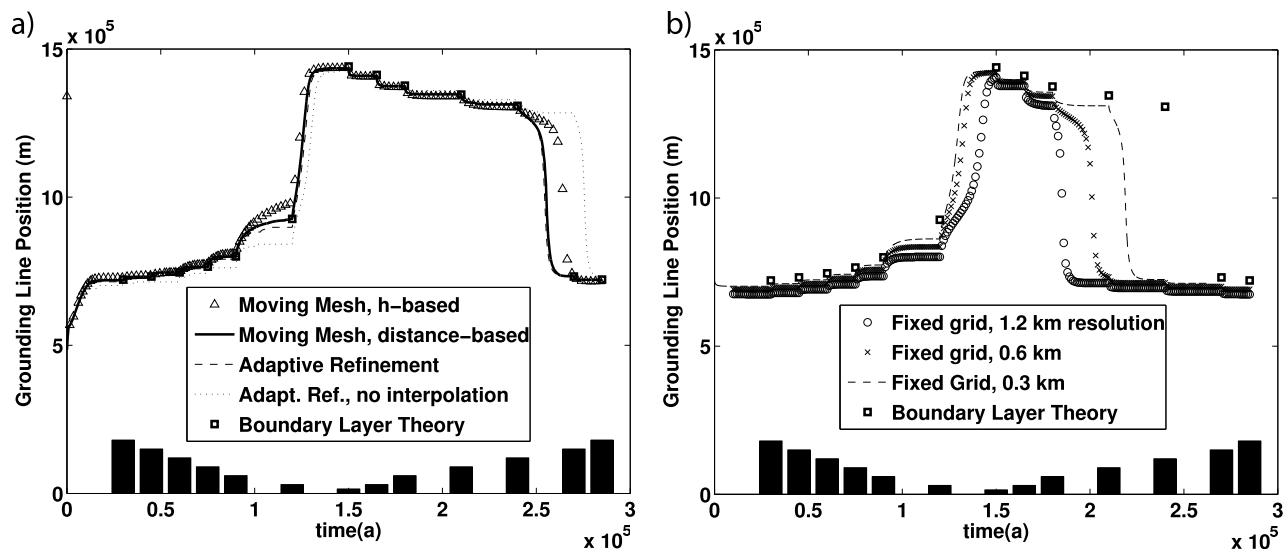
Figure 4. MISMIP experiment 3a: grounding line versus time. Squares represent the steady states predicted by the boundary layer theory. Bars show relative magnitude of Glen's Law constant A for time interval. (a) Moving mesh model and the adaptive refinement model. Solid line and triangles correspond to choices (21) and (22) of the monitor function \omega , respectively. (b) Results without mesh adaption.
