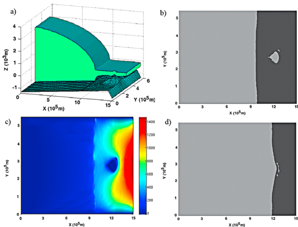
Figure 13. Ice rise experiment. (a) Marine ice sheet with partly grounded shelf (ice rise). The sheet is cut away to reveal the seamount. (b) Domain after 1 ka. Light grey indicates grounded ice, and floating regions are dark. (c) The x -velocity ( \text{ma}^{-1} ) at 1 ka. (d) Domain after 15 ka. The two grounded areas have merged.
