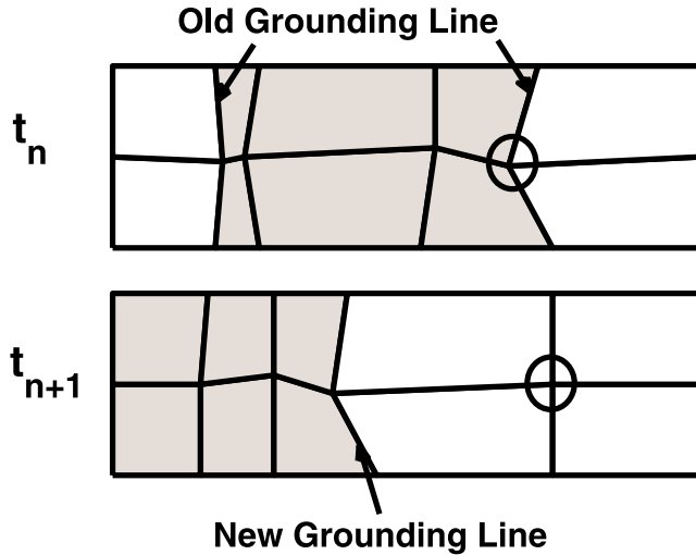
Figure 2. Visualization of moving mesh. (top) A hypothetical mesh at time t_n . (bottom) Mesh at the next time step. In both meshes the shaded cells comprise the grounded domain. Note that the circled node is the same node in both meshes, and it does not remain on the grounding line. Note also that the grounding line can easily change topology; at t_n it is not connected, but at t_{n+1} it is.
