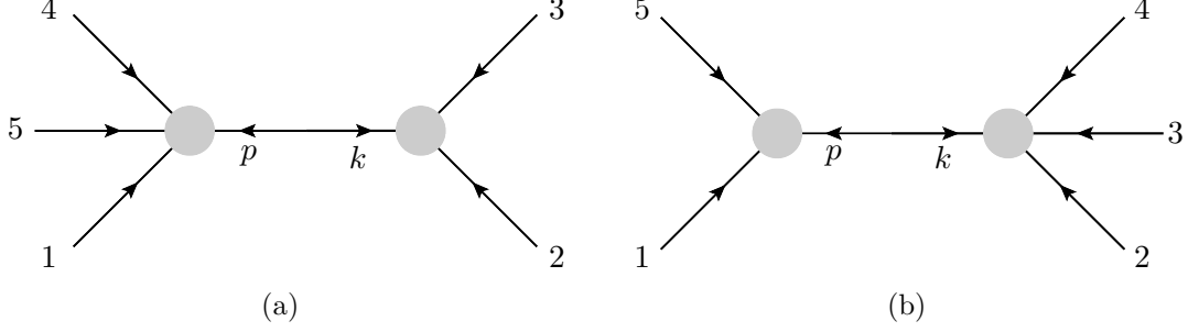
FIG. 2: BCFW diagrams for the five point amplitude.
