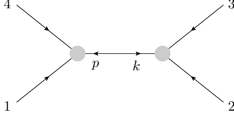
FIG. 1: BCFW diagram for the four point amplitude.
