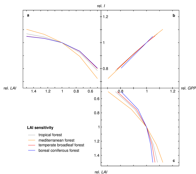
Fig. 3. As in Fig. 1 but varying leaf area index by 25% and 50%.
