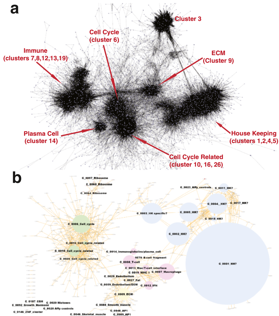
Figure 5 Network graph of conserved transcription signatures in cancer. a) 3D graph layout with labelling of main features in the network's topology. A graph of 9,882 nodes and 184,563 edges was created at Pearson threshold r \geq 0.6 . Clustering of the graph using the MCL algorithm resulted in 639 clusters ranging in size from 1,008 nodes to 4 nodes. A number of large clusters were shown to be highly enriched in genes associated with expression in individual cell types and/or associated with specific cellular functions. See Additional files 3 and 4 for details b) Collapsed cluster diagram showing the conserved gene network as a simplified 2D-network where single nodes represent a gene cluster and are sized according to the number of transcripts within the cluster, edges represent connections between members of each cluster. Nodes representing the main clusters have been coloured according to functional groupings. Blue - clusters represent those associated with housekeeping functions; green - clusters of genes which are directly involved in cell cycle progression or whose expression is in way some linked to it; pink - genes associated with the immune component of the tumour and yellow - other stromal elements. Smaller clusters enriched with genes of known function are also shown.
