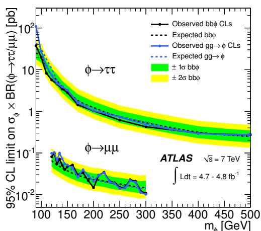
Figure 7. Expected (dashed line) and observed (solid line) 95% CL limits on the cross-section for gluon-fusion and b -associated Higgs boson production times the branching ratio into \tau and \mu pairs, respectively, along with the \pm 1\sigma and \pm 2\sigma bands for the expected limit. The combinations of all \tau\tau and \mu\mu channels are shown. The difference in the exclusion limits obtained for the gluon-fusion and the b -associated production modes is due to the different sensitivity from the b -tagged samples.
