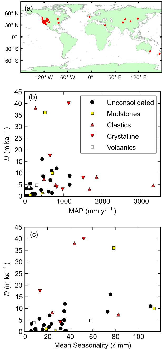
Figure 1. (a) Global distribution of calibrated sediment transport coefficients (red) (Table 1). (b) Mean annual precipitation plotted against calibrated sediment transport coefficients for lithologic groups. In unconsolidated substrate, there is a weak tendency for D to increase with wetter climate ( R^2=0.27 for linear regression). (c) Sediment transport efficiency vs. annual variability of precipitation ( 2\sigma about mean monthly precipitation). D increases with more variable intra-annual precipitation ( R^2=0.51 for linear regression). There were no trends observed when comparing D to mean annual temperature.
