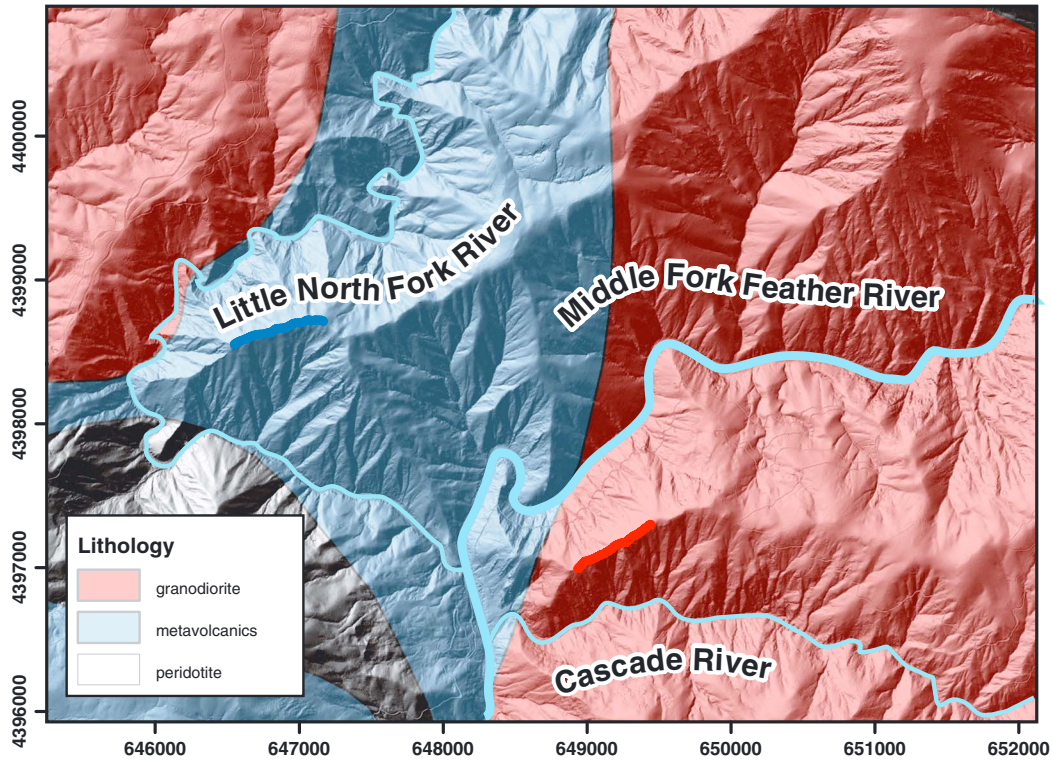
Figure 3. Shaded relief image of study site with lithology superimposed [Moosdorf et al. , 2010]. Topographic metrics from all hillslopes in granodiorite in the east and metavolcanics to the west were retrieved, with more detailed analysis focused on the two ridge transects highlighted in red and blue, respectively. The principle drainage conduits are highlighted in light blue. The spatial reference system is UTM Zone 10N with spatial units in meters.
