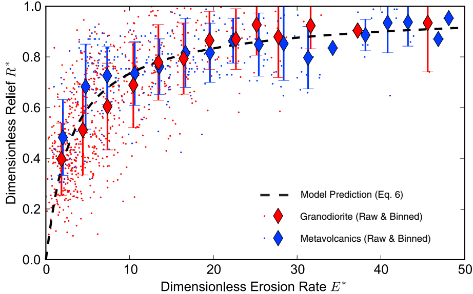
Figure 8. Non-dimensional erosion rate ( E^* ) and relief ( R^* ) calculated from topographic metrics following equations (5b) and (6b) for hilltops in the granodiorite (red) and metavolcanics (blue), using maximum likelihood estimated values for S_C of 0.79 and 0.85, respectively. Data are binned into regularly spaced bins in E^* . Black dashed line shows theoretical relationship predicted by equation (6a) for steadily eroding hillslopes. Non-dimensional analysis effectively normalizes the data from Figure 7 for variation in hillslope length. Hillslopes in the metavolcanics tend to be steeper for a given erosion rate despite correcting for hillslope length, suggesting a greater number of hillslopes undergoing transient adjustment were sampled in the metavolcanics (see text for further discussion).
