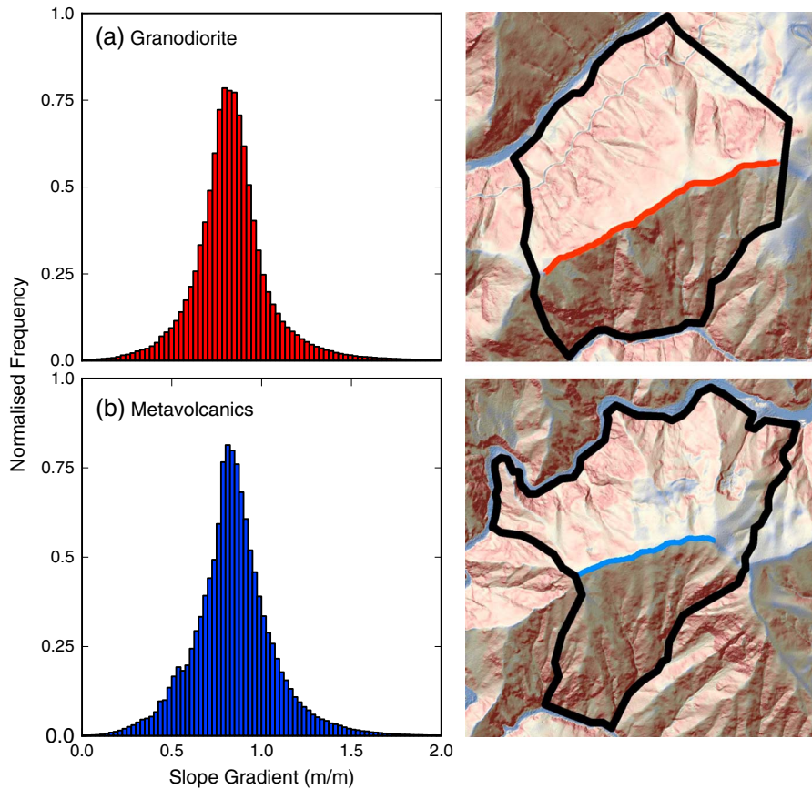
Figure 10. Distribution of hillslope gradients and area sampled for hillslopes in (a) Cascade Pluton and (b) Little North Fork metavolcanics. Slope calculated over 12 m window following Hurst et al. [2012]. For Cascade, mean slope is 0.84 and median slope is 0.83. For the Little North Fork, mean slope is 0.85 and median slope is 0.86.
