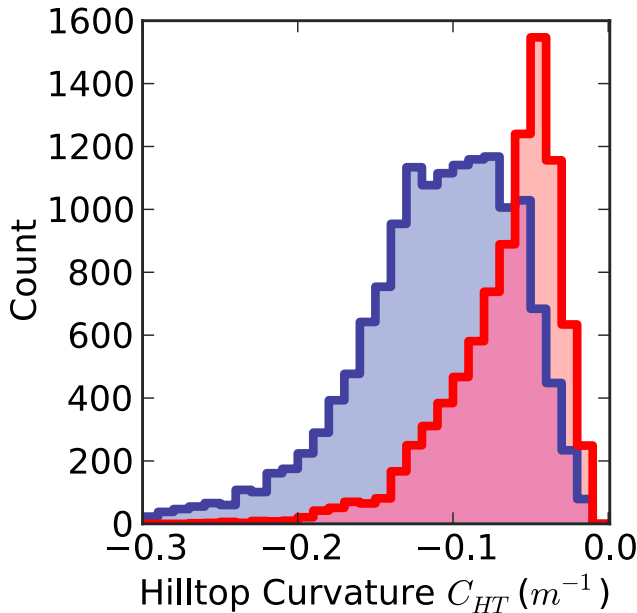
Figure 12. Histogram of hilltop curvatures extracted from hilltops adjacent to the Feather River, Cascade River, and Little North Fork River. Distributions are negatively skewed, and median values (median absolute deviation reported as error range) are -0.105 \pm 0.034 \text{ m}^{-1} and -0.057 \pm 0.019 \text{ m}^{-1} for hilltops in the metavolcanics (blue) and granodiorite (red), respectively.
