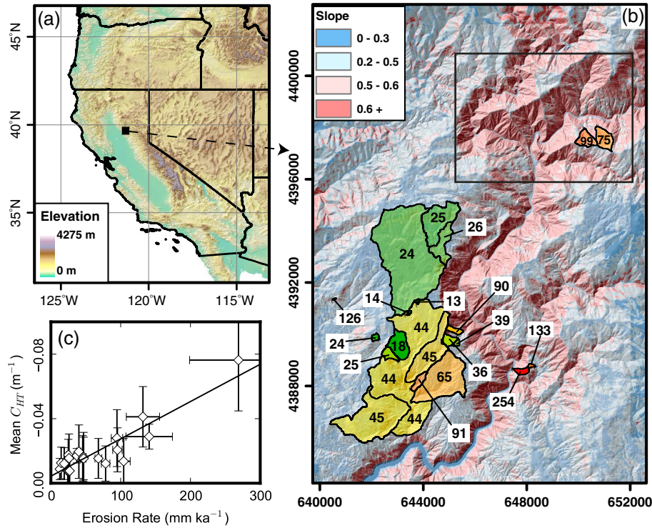
Figure 2. (a) Location of study area in Sierra Nevada of northern California. (b) High resolution (LiDAR) shaded slope map of the study area along the Feather River (Middle Fork); low gradients are blue; steep slopes are red. Overlain are CRN sample sites with estimated basin-averaged erosion rates in mm\ ka^{-1} (shaded green to red with increasing erosion rate, uncertainties on these estimates are shown in (c)) [Hurst et al. , 2012]. Samples were taken for basins exclusively in granitoid bedrock. Erosion rates vary over an order of magnitude from the canyon to the adjacent relict upland. (c) Plot of mean hilltop curvature compared to denudation rate in each of the basins sampled. Solid line represents a linear relationship between hilltop curvature and denudation ( R^2 = 0.83 ), as predicted by equation (4), allowing the sediment transport coefficient to be constrained at 8.6\ m^2\ ka^{-1} [see Hurst et al. , 2012]. The black box shows the location of Figure 3. The spatial reference system is UTM Zone 10N with spatial units in meters.
