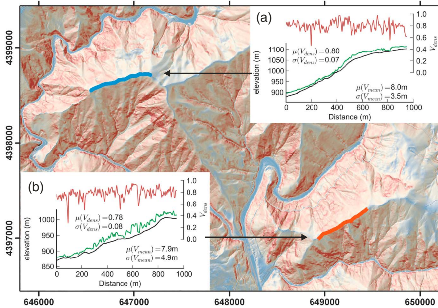
Figure 11. Comparison of vegetation properties for (a) Little North Fork ridge and (b) Cascade Ridge. Vegetation density ( V_{dens} ) is plotted in red, and mean canopy height ( V_{mean} ) is the difference in elevation between the ground surface (black) and mean vegetation elevation (green). Both vegetation parameters are similar between the two sites, but canopy height is more variable on cascade ridge due to the presence of several large trees. Background image is shaded slope map similar to Figure 2. The spatial reference system is UTM Zone 10N with spatial units in meters.
