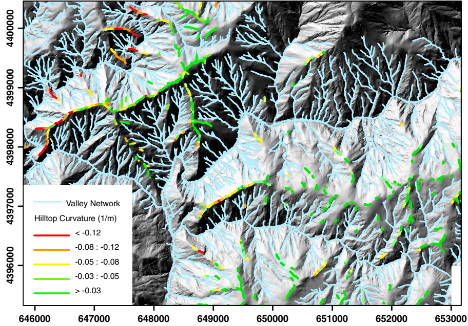
Figure 6. Map of channel and hilltop networks in the study region. Hilltops are color coded by hilltop curvature, with the highest values of hilltop curvature occurring mainly in the metavolcanics and adjacent to the main drainage routes. Channel network extracted using the Geonet tool [Passalacqua et al., 2010]; hilltops defined as the adjoining edges of drainage basins extracted at all stream orders (see text).
