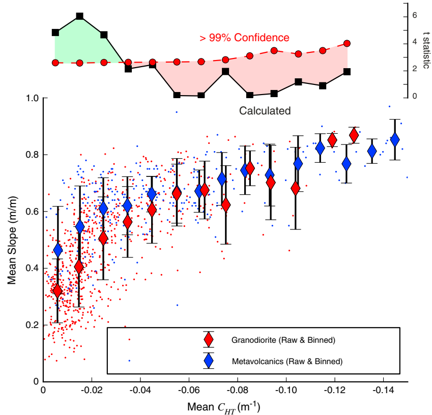
Figure 7. Relationship between mean hilltop curvature ( C_{HT} ) and mean adjacent slope ( S ) for hilltops in the granodiorite (red) and metavolcanics (blue), with Student's t -statistic used to compare between the two datasets. Where the calculated t -statistic (black) falls above the 99% confidence level (red dashed), the two datasets can be interpreted as originating from different populations (area shaded green). Data are binned into regularly spaced bins in C_{HT} . C_{HT} is expected to be a good indicator of relative erosion rate, whilst at high erosion rates, S becomes insensitive to baselevel fall. Note we plot bin-mean averaged C_{HT} and S . In both lithologies, C_{HT} continues to vary despite S becoming limited. For low C_{HT} , hillslopes are steeper in the metavolcanics (at 99% confidence level). S in both lithologies appears to be limited to \sim 0.85 .
