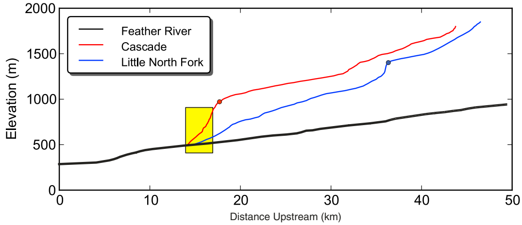
Figure 4. Longitudinal profiles for Little North Fork (blue) and Cascade (red) rivers relative to the lower reaches of the Feather River (black) which sets baselevel. Profiles were generated from U.S. Geological Survey National Elevation Dataset 1/3 arc-second (approx. 10 m) DEMs [http://seamless.usgs.gov/; accessed 15/1/2009]. Shaded region indicates area in which the landscape is interpreted to be adjusting or adjusted to the rapid incision rate of the Feather River along both the Little North Fork and Cascade Rivers, downstream of major knickpoints marked with filled circles. Note these knickpoints both fall out with the bounding region of Figure 3. The lower reaches of Cascade and Little North Fork rivers cross the Cascade Pluton (granodiorite) and Central Belt (metavolcanics), respectively.
