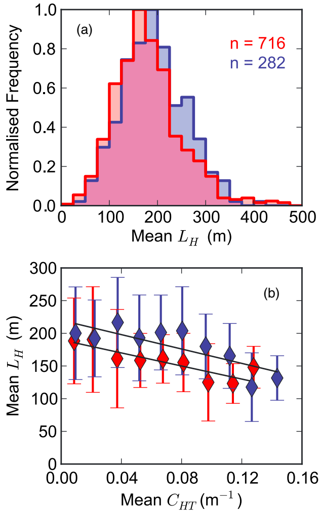
Figure 9. (a) Frequency of hillslope length L_H for the granodiorite (red) and metavolcanics (blue), normalized by the maximum frequency. Maximum frequency occurs at L_H=150\text{--}175 m in the granodiorite and L_H=175\text{--}200 m in the metavolcanics. Additionally, there are more short hillslopes in the granodiorite and more long hillslopes in the metavolcanics. A t -test reveals at 99% confidence that these two datasets are drawn from different populations. (b) Plot of C_{HT} (indicating relative erosion rate) versus L_H in granodiorite (red) and metavolcanics (blue). Black lines represent linear least-square fits to binned averages with R^2=0.74 and 0.66 , respectively. Hillslope lengths tend to shorten with increasing hilltop curvature (an indicator of erosion rates).
