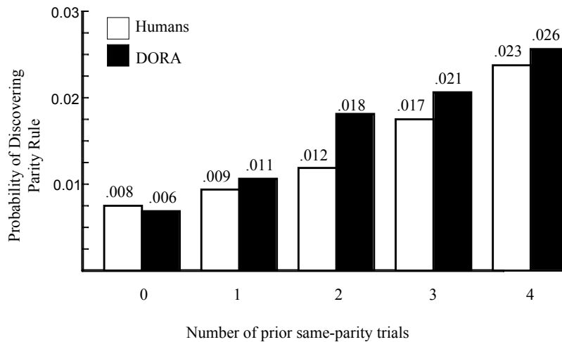
Figure 15. Simulation of Dixon and Bangart’s (2004) data.
