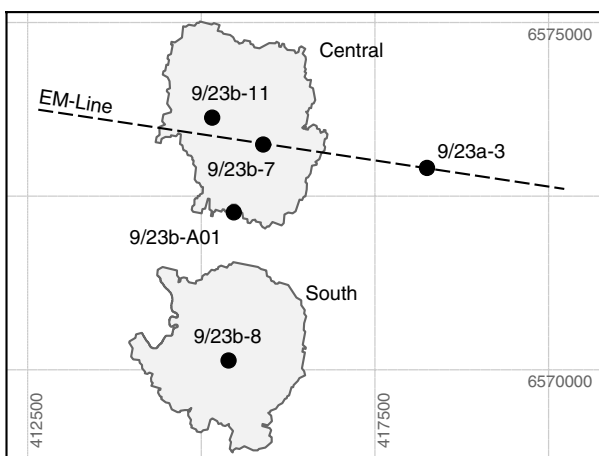
Figure 5. Location of Harding Central and Harding South, the EM survey outlines from 2007 and 2008, and the five wells we use in our example. Well 9/23b-8 is our calibration well. Wells 9/23b-7, 9/23b-11, 9/23b-A01, and 9/23a-3 are our control wells, where the ultimate one is off-target.
