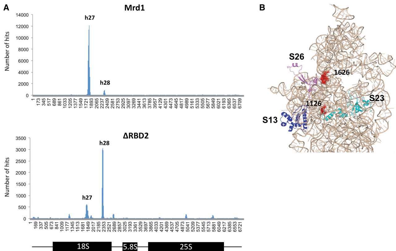
Figure 5. RBD2 is important for Mrd1 association with h27. (A) High-throughput sequencing of CRAC cDNA library for wt Mrd1 and \Delta RBD2. Histogram shows hits (y-axis) versus the position in 35S pre-rRNA (x-axis). h27 and h28 are denoted. (B) The modelled Mrd1 binding sites (red) of nucleotides 1126 and 1626 are located and highlighted in the mature secondary structure of S. cerevisiae 18S rRNA. The location of small ribosomal subunit proteins S13 (blue), S23 (light blue) and S26 (purple) are indicated as references.
