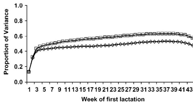
Figure 7. Proportion of total phenotypic variance of total body energy content in second (□) and third (◇) lactations predicted from weekly first-lactation animal genetic evaluations.
