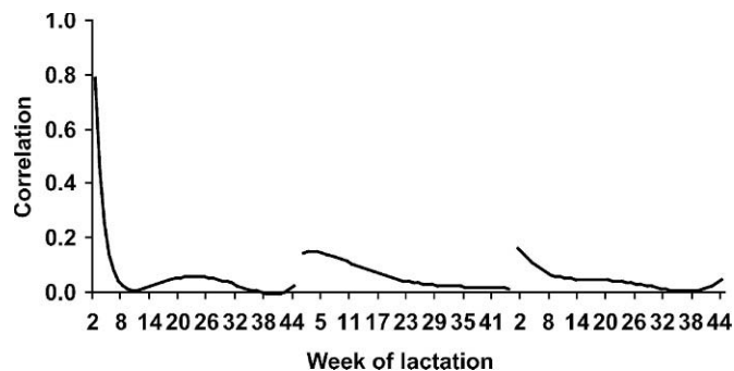
Figure 3. Estimated genetic correlation between total body energy content in wk 1 of first lactation and later weeks of all 3 lactations.
