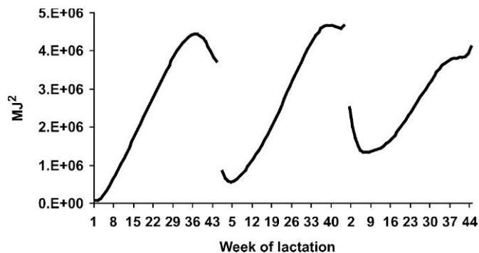
Figure 2. Estimated genetic variance of total body energy content by week in the first 3 lactations (SE lactation 1 = 51,800 to 184,700 MJ 2 ; SE lactation 2 = 90,430 to 345,600 MJ 2 ; SE lactation 3 = 100,900 to 368,300 MJ 2 ).
