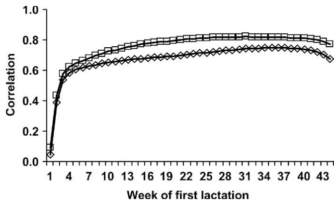
Figure 6. Estimated genetic correlation between total body energy content in the 44 wk of first lactation and wk 13 (week of minimum body energy content) in second (□) and third (◇) lactations.
