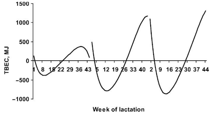
Figure 1. Least square mean phenotypic values of total body energy content (TBEC) by week in the first 3 lactations.
