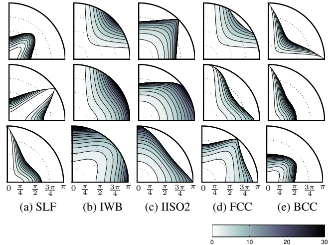
Figure 8: Volumetric slices of wave speed error as a function of polar angle \theta \in [0, \pi/2] on a plane and radius \omega_k \in (0, \pi] with 2% error contours. First row: \xi_z = 0 plane, second row: \xi_x = \xi_z plane, third row: the plane described by the zero point and the normal vector \hat{n} = (1, 1, 1) .
