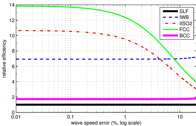
Figure 10: Efficiency for FD schemes relative to SLF.
