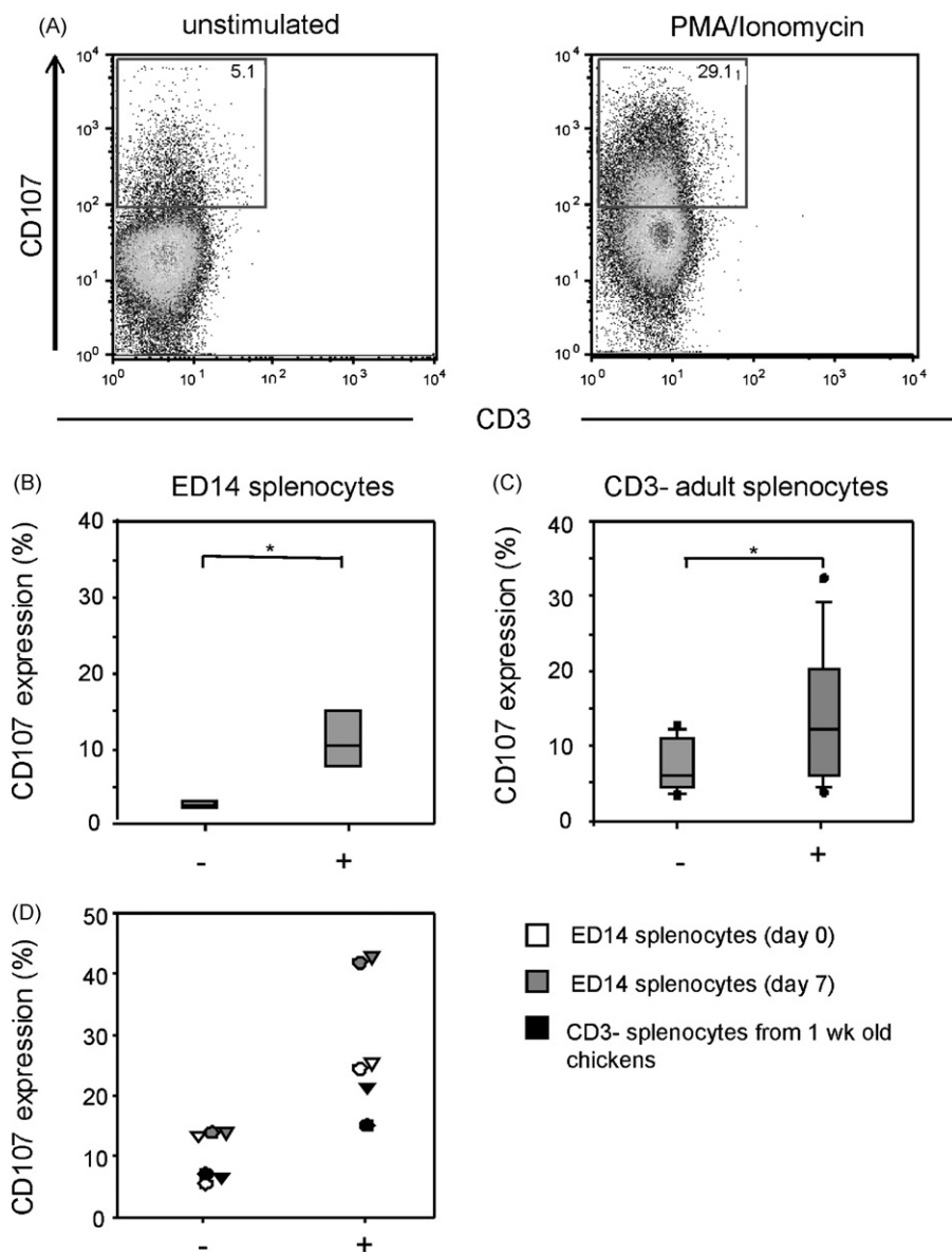
Fig. 4. Expression of ChCD107 (LAMP-1) can be used to measure activation of chicken NK-cells. (A) Embryonic and adult splenocytes were stimulated with PMA/Ionomycin for 4 h and CD107 expression was analysed by flow cytometry. A representative example of CD107 expression in the absence (left panel) and presence (right panel) of stimuli is shown. (B) Stimulation of embryonic splenocytes directly ex vivo resulted in a significant increase in CD107 expression ( n = 5 ). (C) Stimulation of splenocytes with PMA/Ionomycin results in a significant increase in CD107 expression in CD3 - splenocytes ( n = 12 ). (D) Co-incubation of splenocytes with the chicken B-cell-line LSCC-RP-9 (NK target cell-line) results in an increase in CD107 expression in NK-cells from different sources ( n = 6 ). Significant differences ( p < 0.05 ) are indicated by an asterisk.
