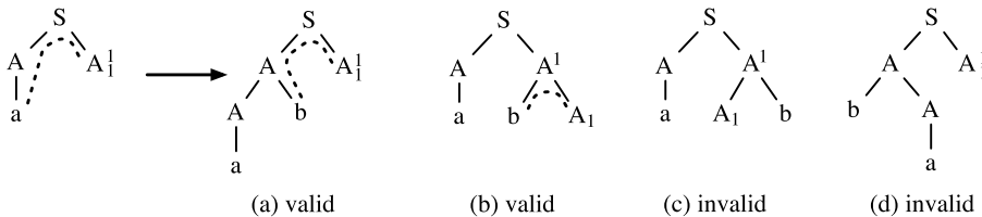
Figure 7 Adjunction in an incremental derivation. Only adjunction of auxiliary trees with leftmost foot nodes into upward visits of the current fringe (a) or with rightmost foot nodes into downward visits (b) result in valid prefix trees; the other two combinations are invalid (c, d).
