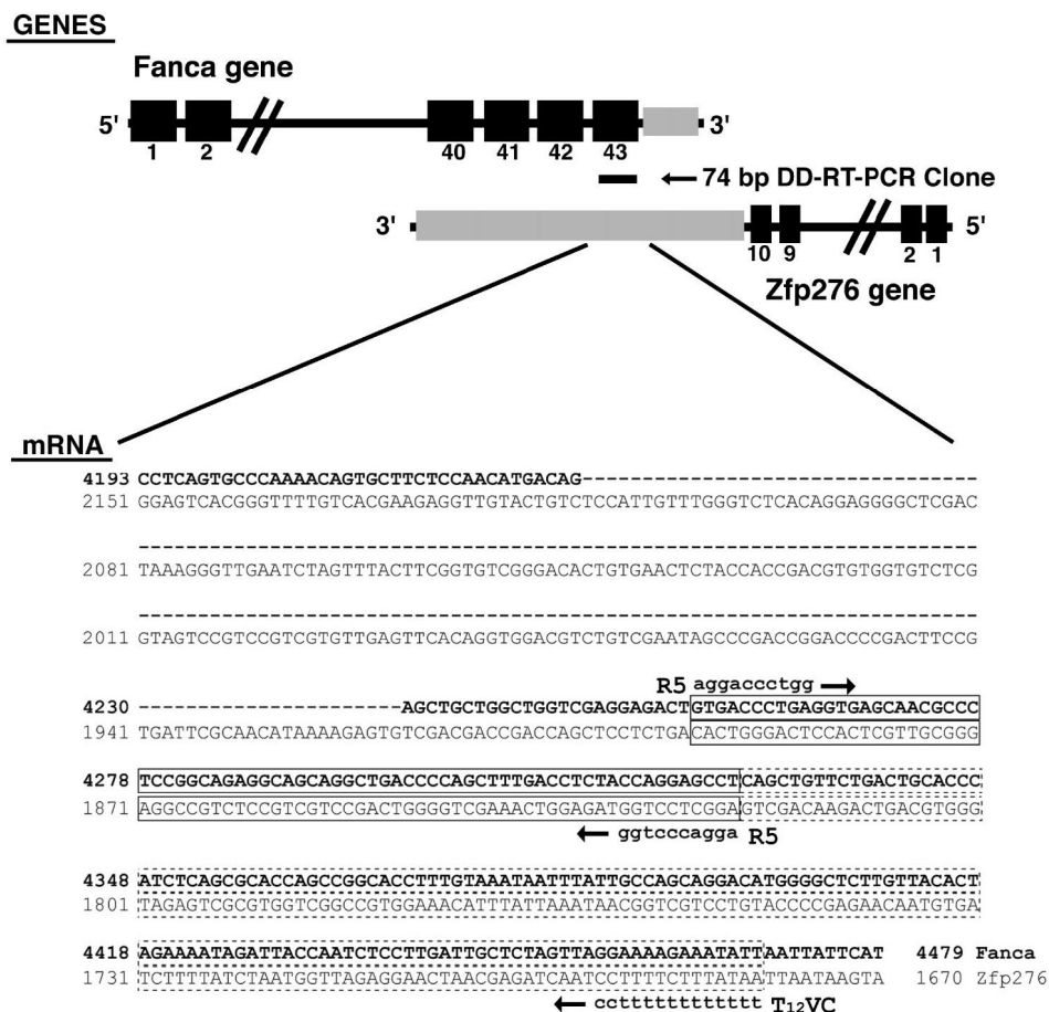
FIG. 2. Schematic representation of the Fanca locus showing the location of the differential display RT-PCR clone. Exons 40-43 of Fanca , shown as black boxes, overlap with the 3' untranslated region (UTR) of Zfp276 , shown in grey. The location of the cloned 74-bp differential display (DD) RT-PCR clone is indicated. Beneath the schematic, the regions of nucleotide identity between Fanca mRNA and Zfp276 mRNA have been aligned, Fanca mRNA sequence is shown in bold type, and spliced intronic sequence has been omitted and replaced with a dashed line, with Zfp276 mRNA in normal typeface. The amplified 74-bp DD-RT-PCR clone has been boxed with a solid line, and the original 216-bp DD-RT-PCR clone is indicated as an extension of the boxed region with dashed lines. The amplification primers R5 and T 12 VC are also shown on the corresponding Fanca sequence. No suitable priming sites were identified by bioinformatic analysis for the T 12 VC-anchored primer on the Zfp276 3' UTR sequence.
