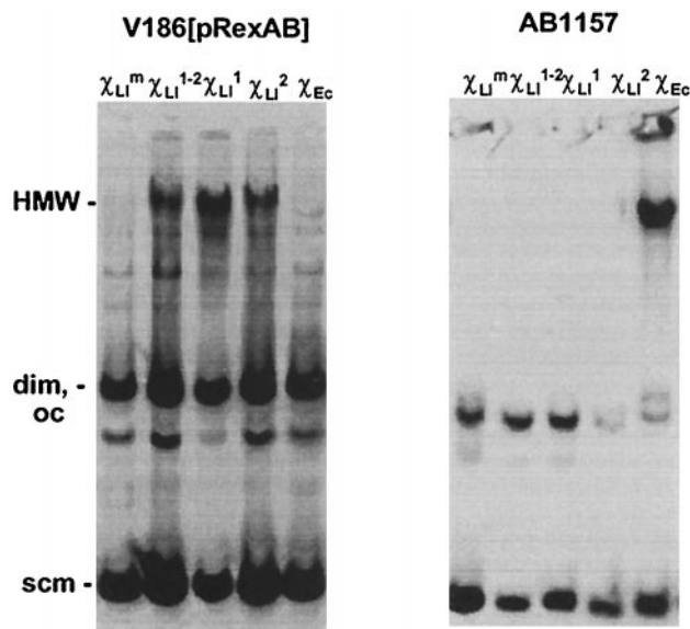
FIG. 3. \text{Chi}_{\text{LI}} is specifically recognized by RexAB. E. coli strains containing plasmid pRC2 with \text{Chi}_{\text{LI}} or \text{Chi}_{\text{EC}} were grown to mid-logarithmic phase, and whole-cell lysates were prepared. HMW was detected by Southern hybridization by using pRC2 as probe. Plasmids are: pRC2- \text{Chi}_{\text{LI}}^{\text{m}} (containing mutated \text{Chi}_{\text{LI}} , \chi_{\text{LI}}^{\text{m}} lanes), pRC2- \text{Chi}_{\text{LI}}^{1-2} (containing head-to-head copies of \text{Chi}_{\text{LI}} , \chi_{\text{LI}}^{1-2} lanes), pRC2- \text{Chi}_{\text{LI}}^1 (containing \text{Chi}_{\text{LI}} in orientation 1, \chi_{\text{LI}}^1 lanes), pRC2- \text{Chi}_{\text{LI}}^2 (containing \text{Chi}_{\text{LI}} in orientation 2, \chi_{\text{LI}}^2 lanes), pRC2- \text{Chi}_{\text{EC}}^2 (containing \text{Chi}_{\text{EC}} in orientation 2, \chi_{\text{EC}} lanes). Smear and bands below HMW in V186[pRexAB] strain appear to be secondary products of HMW accumulation.
