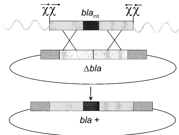
FIG. 4. Strategy to test \text{Chi}_{\text{LI}} effect on RexAB-mediated recombination. Linear transforming DNA contains an internal fragment of bla ( \text{bla}_{\text{int}} , solid rectangle) and has an additional 360 bp flanking homology with bla (grey rectangle). Double Chi sites on the linear fragments, (either \text{Chi}_{\text{LI}} or \text{Chi}_{\text{EC}} ) oriented for recognition to enhance recombination, are represented by \chi\chi . Wavy lines represent heterologous dsDNA tails. Plasmid p \Delta\text{Bla} bears an internal deletion of bla ( \Delta\text{bla} ), the target for gene conversion. Hatched rectangles represent ends of the bla gene not present on linear DNA. Double crossover homologous recombination would be required to convert cells to Amp r ( \text{bla}^+ ).
