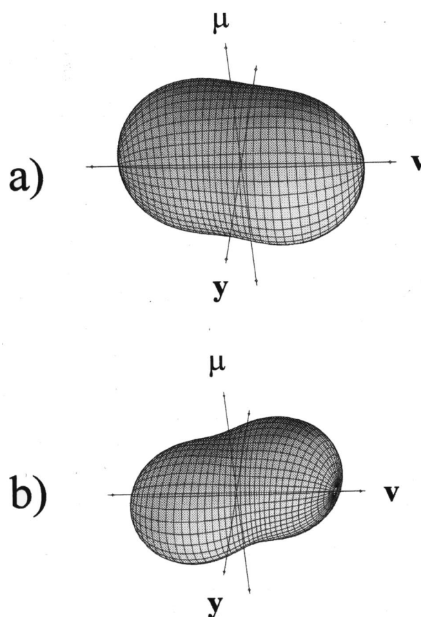
FIG. 9. (a) Plot of the complete angular momentum distribution for the ^{37}\text{Cl} photofragments from the photodissociation of ICl at 516 nm and (b) 510 nm. The photolysis polarization lies 45^\circ to the recoil direction.
