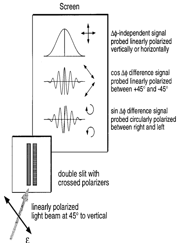
FIG. 10. Variant of Young's double-slit experiment. The light beam is initially linearly at 45^\circ to vertical, and crossed polarizers are placed in front of the two slits, producing a polarization interference pattern on the screen. The polarization pattern can be probed with linear and circular polarizers. The pattern at top is produced when a linear polarizer is placed either vertically or horizontally in front of the screen, and is \Delta\phi independent (analogous to the incoherent alignment parameters). The pattern in the middle is the difference between patterns produced by a linear polarizer placed at 45^\circ and separately at -45^\circ to vertical, and varies as \cos \Delta\phi (analogous to \text{Re}[\mathbf{a}_1^{(2)}(\parallel, \perp)] ). The pattern at the bottom is the difference between patterns produced by right and left circular polarizers, and varies as \sin \Delta\phi (analogous to \text{Im}[\mathbf{a}_1^{(1)}(\parallel, \perp)] ).
