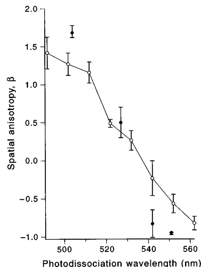
FIG. 3. Measurement of the Cl-photofragment spatial anisotropy parameter \beta from the photodissociation of ICI with linearly polarized light in the 490–560 nm range (open circles). Notice that this parameter ranges from close to the limiting values of \beta = +2 at 490 nm to \beta = -1 at 560 nm. This indicates that the dissociation of ICI proceeds predominantly via a parallel transition (through the B state) at 490 nm and predominantly via a perpendicular transition (through the A state) at 560 nm. The dark circles are predictions of the spatial anisotropy parameter derived from the envelope of the oscillations of the \text{Im}[\mathbf{a}_1^{(1)}(\parallel, \perp)] parameter (see text).
