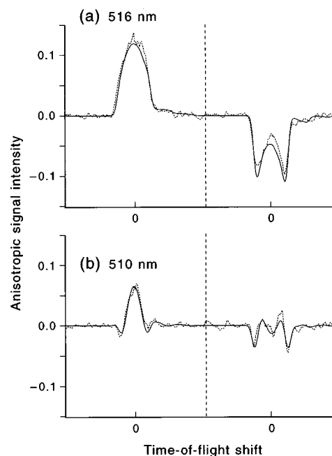
FIG. 5. (a) The anisotropic profiles I_{\text{aniso}}^X and I_{\text{aniso}}^Z of the ^{37}\text{Cl} photofragments from the photodissociation of ICl at 516 nm and (b) 510 nm. These pairs of composite profiles are sensitive to the complete alignment of the ^{37}\text{Cl} photofragment angular momentum distributions described by the four polarization parameters of k=2 (see text). Notice how dramatically the anisotropic signals sensitive to photofragment alignment change between photodissociation wavelengths of 516 and 510 nm, in strong contrast to the isotropic signals shown in Fig. 4.
