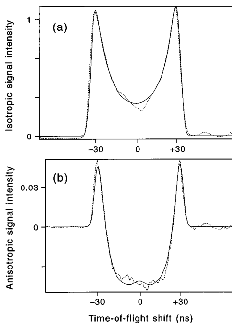
FIG. 2. (a) The isotropic ^{35}\text{Cl}^+ ion-arrival composite profile, \mathbf{I}_{\text{iso}}^x , from the photodissociation of \text{Cl}_2 at 320 nm, which is sensitive to the Cl-photofragment speed distribution. The photolysis polarization lies perpendicular to the time-of-flight axis. This profile shows that the spatial anisotropy of the photofragments is well described by the pure-perpendicular transition limiting value of \beta = -1 . (b) The anisotropic profile, \mathbf{I}_{\text{aniso}}^x , is sensitive to the complete Cl-photofragment angular momentum distribution described by the \mathbf{a}_0^{(2)}(\perp) and \mathbf{a}_2^{(2)}(\perp) parameters only. Analysis of these profiles yields \mathbf{a}_0^{(2)}(\perp) = -0.50 and \mathbf{a}_2^{(2)}(\perp) = -0.32 , indicating that the photofragment angular momentum distribution is not cylindrically symmetric about the recoil direction.
