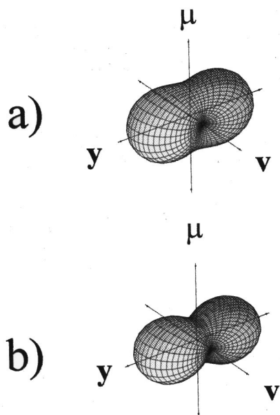
FIG. 8. (a) Plots of the Cl-photofragment angular momentum distributions from the photodissociation of \text{Cl}_2 at 320 nm. Notice that the J=3/2 angular momentum is strongly peaked perpendicular to both the recoil direction \hat{\mathbf{v}} and the transition dipole moment \mu . (b) A plot of the m_y = \pm 3/2 distribution, showing the strong similarity with the experimental measurement, and that the measured Cl atoms are nearly maximally aligned with respect to the y axis.
