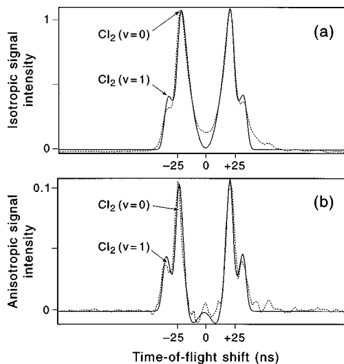
FIG. 1. (a) The isotropic core-extracted 35 Cl + ion-arrival composite profile, I_{\text{iso}}^Z , from the photodissociation of Cl 2 at 470 nm, which is sensitive to the Cl photofragment speed distribution. The photolysis polarization lies along the time-of-flight axis. Notice the fast photofragments from the photodissociation of v=1 Cl 2 , and the slower photofragments from the photodissociation of v=0 Cl 2 . (b) The anisotropic core-extracted profile, I_{\text{aniso}}^Z , is sensitive to the Cl-photofragment angular momentum distributions. These distributions are described by the \mathbf{a}_0^{(2)}(\parallel) parameter, and analysis of these profiles yields \mathbf{a}_0^{(2)}(\parallel) \approx -0.7 for both channels.
