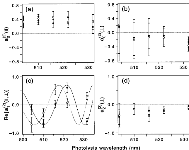
FIG. 6. The 504–532 nm wavelength dependence of the a_0^{(2)}(||) , a_0^{(2)}(\perp) , \text{Re}[a_1^{(2)}(||, \perp)] , and a_2^{(2)}(\perp) parameters describing the complete ^{35}\text{Cl} and ^{37}\text{Cl} photofragment alignment from the photodissociation of ICl (shown by the dark and open circles respectively). Notice that, within experimental error, the three incoherent contributions to the alignment, the a_0^{(2)}(||) , a_0^{(2)}(\perp) , and a_2^{(2)}(\perp) parameters, are approximately constant as a function of dissociation wavelength. In sharp contrast, the coherent contribution to the photofragment alignment, the \text{Re}[a_1^{(2)}(||, \perp)] interference term, vary dramatically. The solid and dashed lines are the predictions of \cos \Delta\phi for ^{35}\text{Cl} and ^{37}\text{Cl} , respectively, offset by -2 nm (see text). The agreement between the oscillations of \text{Re}[a_1^{(2)}(||, \perp)] and \cos \Delta\phi are excellent.
