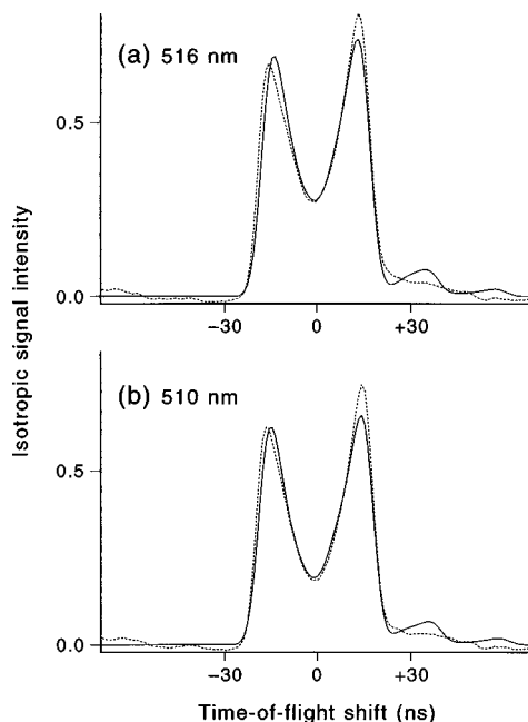
FIG. 4. (a) The isotropic ^{37}\text{Cl}^+ ion-arrival composite profile, I_{\text{iso}}^Z , from the photodissociation of ICl at 516 nm and (b) at 510 nm. Notice that the profiles are very similar; the profile at 510 nm is somewhat more dipped in the center than the profile at 516 nm, as \beta at this frequency is somewhat more positive. Other than this, there are no large changes in the speed distribution.
