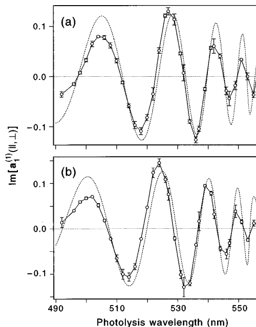
FIG. 7. The 490–560 nm wavelength dependence of the \text{Im}[a_1^{(1)}(||, \perp)] parameter describing the (a) ^{35}\text{Cl} and (b) ^{37}\text{Cl} photofragment orientation from the linearly polarized photodissociation of ICl. The dashed lines are the predictions of \sin \Delta\phi for ^{35}\text{Cl} and ^{37}\text{Cl} (see text); the amplitude of the \sin \Delta\phi plots are multiplied by an envelope calculated from the spatial anisotropy measurements shown in Fig. 3. The actual, more pronounced, experimental envelope is inverted to predict \beta as a function of wavelength as discussed in the text and shown in Fig. 3.
