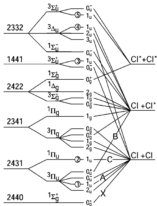
FIG. 4. Correlation diagram showing all of the electronic states of \text{Cl}_2 , (Refs. 2 and 3). On the right-hand side ground-state \text{Cl}(^2P_{3/2}) and excited-state \text{Cl}^*(^2P_{1/2}) are denoted as \text{Cl} and \text{Cl}^* , respectively, as in the text. The left-hand side shows the electronic configuration of the molecular orbitals 5\sigma_g 2\pi_u 2\pi_g^* 5\sigma_u^* . The electronic terms are shown along with the projection of total electronic angular momentum, \Omega . The five states of \Omega=1_u symmetry that are important for the present discussion are labeled in energetic order from 1 to 5, as they are in the text, e.g., 1_u^{(1)} is the lowest state ( A state). States X , A , B , and C are also highlighted for convenience.
