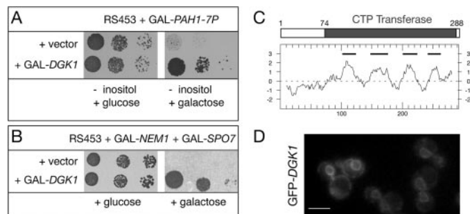
FIGURE 2. DGK1 rescues the lethality of dephosphorylated PAH1 . A , identification of DGK1 as a high copy suppressor of the inositol auxotrophy of PAH1-7P . The wild-type RS453 strain carrying a high copy vector expressing the non-phosphorylated PAH1-7P mutant from a galactose-inducible promoter was transformed with the indicated plasmids. Transformants were grown on synthetic plates lacking inositol and supplemented with glucose ( left panel ) or galactose ( right panel ) at 30 °C. B , identification of DGK1 as a high copy suppressor of the lethality of NEM1-SPO7 overexpression. RS453 cells carrying plasmids coexpressing NEM1 and SPO7 from a galactose-inducible promoter were transformed with the indicated plasmids. Transformants were grown on synthetic plates supplemented with glucose ( left panel ) or galactose ( right panel ) at 30 °C. C , primary structure and hydropathy plot of Dgk1p. The gray box indicates the conserved cytidylyltransferase domain within Dgk1p. Below, the hydropathy plot of Dgk1p is given (42), using a window of 19 amino acids. The black lines indicate the positions of the predicted transmembrane domains. D , GFP-Dgk1p localizes to the nuclear membrane and ER. A GFP-DGK1 fusion under the control of the DGK1 promoter was expressed from a centromeric plasmid in a dgk1Δ strain. Cells were grown in early logarithmic phase and visualized by fluorescent microscopy. Scale bar = 5 \mu m.
