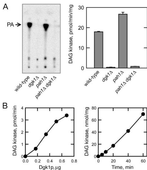
FIGURE 5. Dgk1p is a novel CTP-dependent DAG kinase. A, the dgk1Δ mutation abolishes diacylglycerol kinase activity. Cell extracts were prepared from wild-type, dgk1Δ , pah1Δ , and pah1Δ dgk1Δ cells at the exponential phase of growth, and 50 \mu\text{g} of protein from each cell extract was assayed for diacylglycerol kinase activity. Left panel, the ^{32}\text{P} -labeled reaction product was extracted with chloroform, separated by thin layer chromatography using a solvent system of chloroform/methanol/water (65:25:4), and visualized by phosphorimaging. Right panel, the ^{32}\text{P} -labeled reaction product was extracted with chloroform and subjected to liquid scintillation counting. Each data point represents the mean \pm S.D. of triplicate enzyme determinations. B, Dgk1p exhibits DAG kinase activity. The DAG kinase activity of partially purified Dgk1p was measured with the indicated protein content (left panel) and for the indicated time intervals (right panel).
