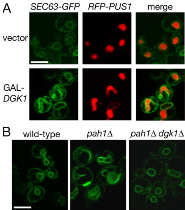
FIGURE 3. DGK1 opposes the function of PAH1 at the nuclear membrane. A , overexpression of DGK1 causes nuclear/ER membrane proliferation and nuclear expansion. The RS453 strain expressing the plasmid-borne SEC63-GFP and RFP-PUS1 reporters was transformed with a centromeric plasmid expressing DGK1 under the control of a galactose-inducible promoter or an empty vector. Cells were grown in galactose-containing medium and visualized by confocal microscopy. Scale bar = 5 \mu m. B , deletion of DGK1 restores normal nuclear structure in pah1 \Delta cells. Wild-type RS453, pah1 \Delta , and pah1 \Delta dgk1 \Delta cells transformed with a centromeric plasmid expressing SEC63-GFP were visualized by confocal microscopy. Scale bar = 5 \mu m.
