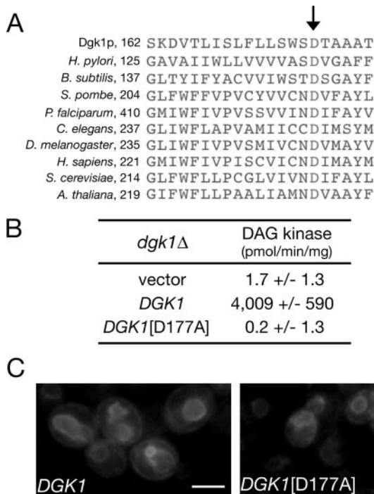
FIGURE 6. The DAG kinase activity of Dgk1p is required for nuclear membrane expansion. A , multiple sequence alignment of Dgk1p (residues 162–182) with cytidyltransferases from the indicated species. The first residue of each sequence segment is indicated. The arrow points to the conserved aspartate residue. B , the DGK1 (D177A) mutant lacks DAG kinase activity. The dgk1 Δ strain was transformed with an empty centromeric plasmid or with the same plasmid carrying DGK1 or DGK1 (D177A) under the control of the GAL1/10 promoter. Cell extracts from the corresponding strains were assayed for diacylglycerol kinase activity. Values and errors were calculated from three experiments. C , DGK1 (D177A) does not promote nuclear membrane growth. The RS453 strain expressing a SEC63 -GFP fusion was transformed with the galactose-inducible DGK1 or DGK1 (D177A) construct from B , grown to early logarithmic phase in galactose-containing medium, and inspected by microscopy.
