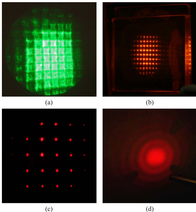
Fig. 2. (Color online) Photographs of (a) the lenslet array illuminated by the pump beam, (b) the active fluorescing regions within the LC, (c) the laser array emission, and (d) the interference fringes obtained when recombining the multiple laser emission sources (Cell A, monodomain sample).
