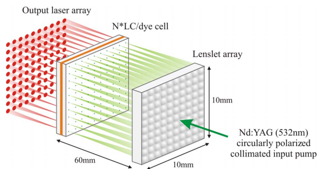
Fig. 1. (Color online) Illustration of the principle for photopumping an LC sample using a lenslet array that generates a diverging output laser array.
