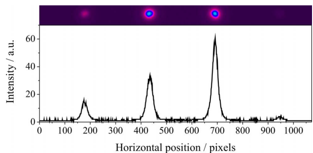
Fig. 3. (Color online) (top) Two-dimensional intensity profiles of the LC laser array emission for a typical row in the array, and (bottom) the corresponding cross section through the data (Cell A, monodomain sample).
