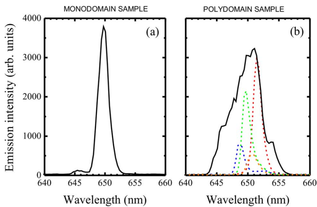
Fig. 4. (Color online) Emission spectra of two different LC laser array samples: (a) Cell A (monodomain sample), all individual laser sources are virtually identical, and the emission can be recombined to give an almost monomode output. (b) Cell B (polydomain sample), (broken curves) multiple monomode sources are achieved each arising from a different domain and chiral pitch (solid curve) and recombination of the laser array results in a broadband emission.
