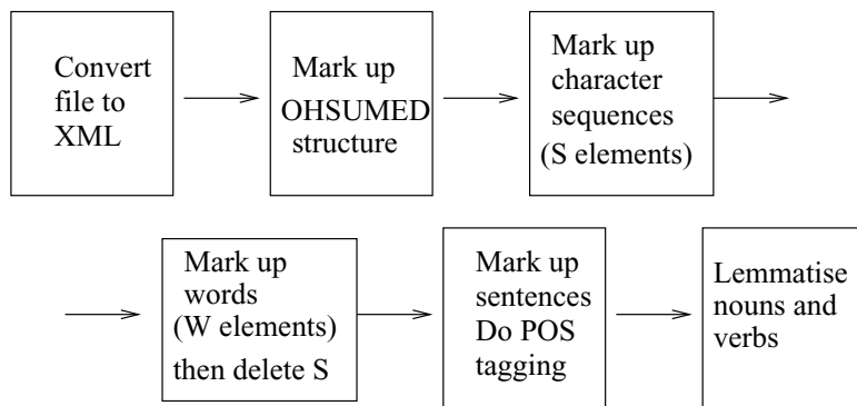
Fig. 3. Pipeline architecture.
