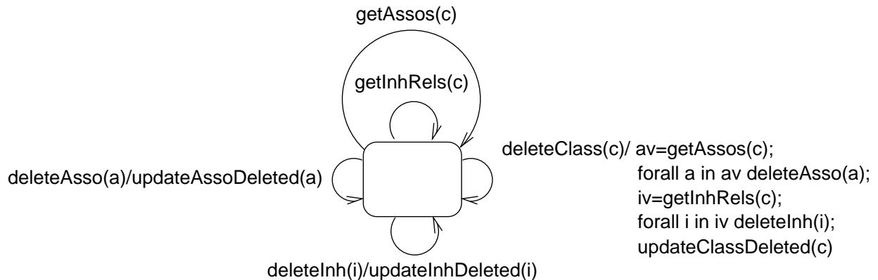
Fig. 6. State machine for Model
