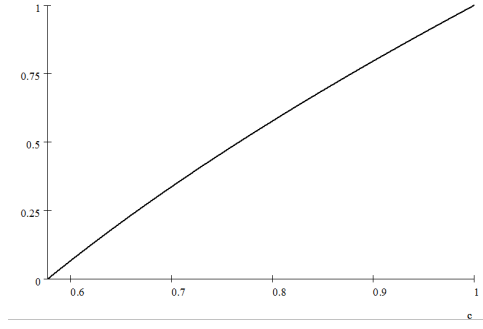
Figure 9: Condition 53 as a function of c assuming a uniform distribution of talent
