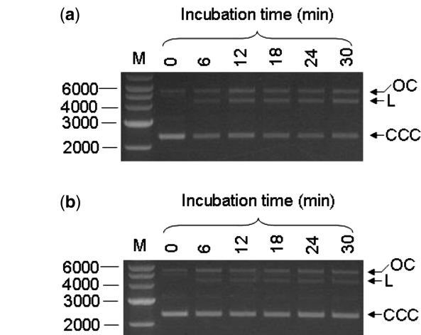
Figure 2. The effect of extended reaction times for ratios of EcoKI to DNA of 0.6:1 (a) and 0.4:1 (b). The concentration of plasmid pBRsk1 was 3 nM. The leftmost lane is a DNA size ladder as in Figure 1. The following lanes show time points of 0, 6, 12, 18, 24 and 30 min digestion. The reactions are complete within 6–12 min as no further increase in L DNA is seen at later times.
