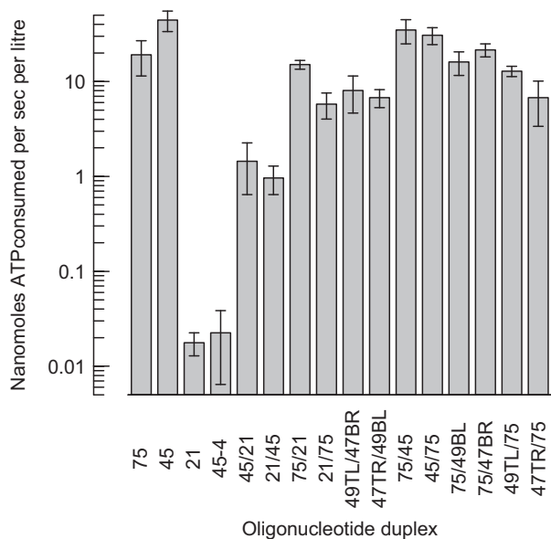
Figure 6. ATP hydrolysis activity of EcoKI on various oligonucleotide duplexes as measured using the NADH-coupled enzyme assay. The assay contained 10 nM EcoKI, 5 nM of the appropriate DNA duplex given in Table 1, 0.1 mM SAM and 2 mM ATP.
