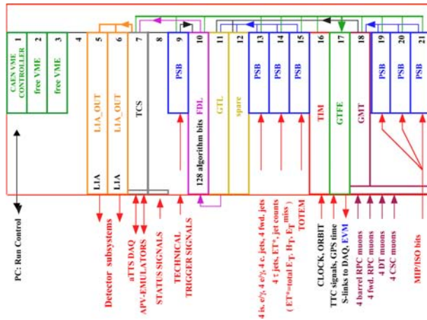
Figure 8.7: Global Trigger central crate.
