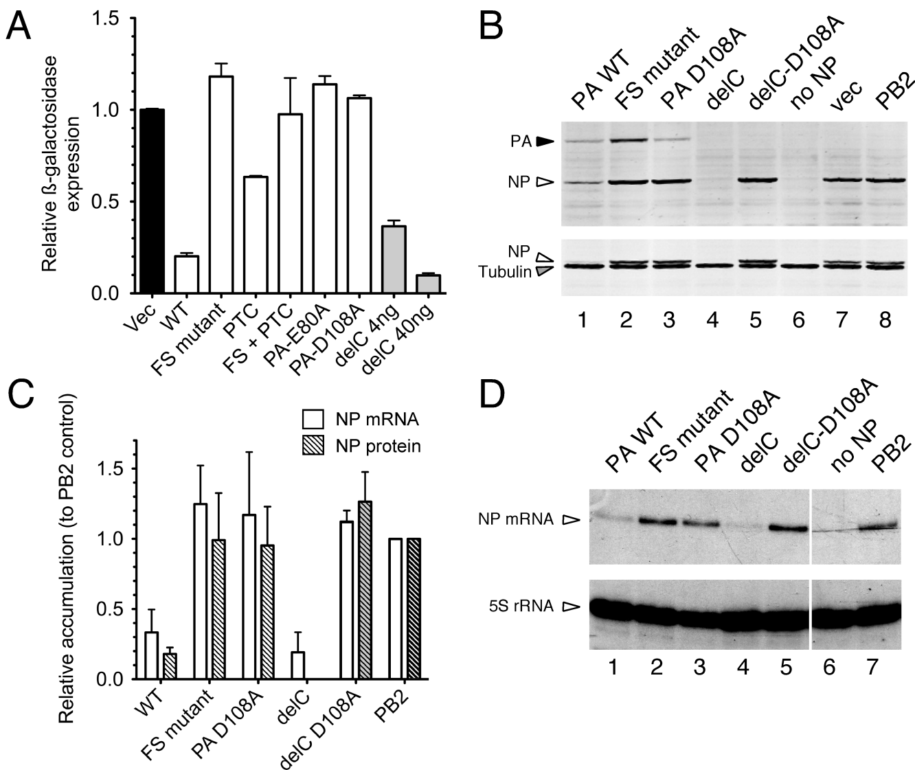
Fig. 2. PA-X mediated repression of plasmid-driven gene expression
