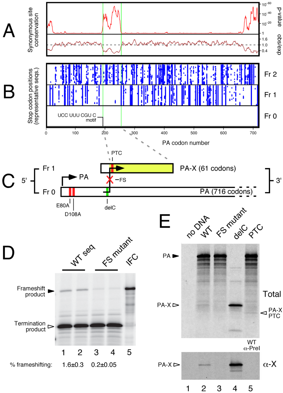
Fig. 1. Characterization of a ribosomal frameshift signal in IAV segment 3
