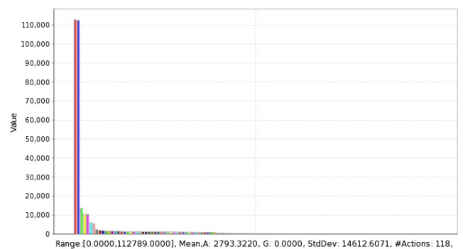
Figure 3: Number of occurrences observed in a trace as reported by Traviando.
