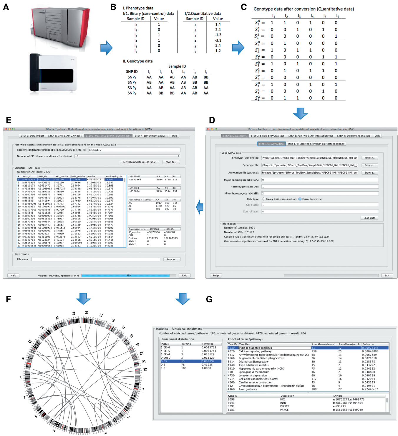
Figure 1. BiForce Toolbox workflow. GWAS data are generated by microarray or next-generation sequencing platforms (A). Example of input data formats for disease and quantitative traits (B). Example of genotype data conversion and storage in bitwise arrays (C). Snapshot of the BiForce Toolbox GUI after loading and conversion of the BMI data of the NFBC1966 cohort (note the multi-tab options such as working with subsets of SNPs or SNP-pairs and performing single SNP-based genome-wide association) (D). Snapshot of the BiForce Toolbox GUI running the pairwise genome scan of the BMI data with progress reporting at the bottom (note SNP information, genotype counts, contingency table are shown for a retained pair of SNPs; the retained results of the pairwise genome scan can be exported as tab-separated text file or Excel compatible spreadsheet for further analyses by users) (E). A graphic view of positions of interaction signals in BMI of the NFBC1966 cohort generated by a third party tool Circoos, where chromosome ideograms are shown around the outer ring and are oriented pter-qtter in a clockwise direction with centromeres indicated as red bands (F). Snapshot of the BiForce Toolbox GUI running pathway enrichment analysis after the pairwise genome scan using epistatic genes with interaction -\log_{10} P values greater than 7.3 (i.e. P < 5.0e^{-08} ; note the member epistatic genes and associated SNPs are displayed for a pathway selected) (G).
