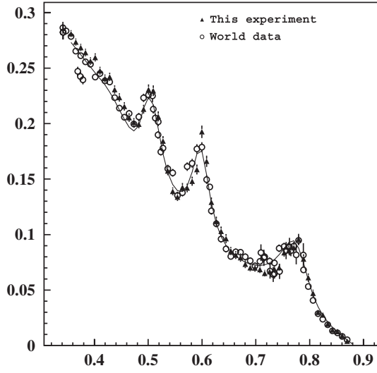
FIG. 7. Inclusive structure function F_2 at Q^2 = 2 ( \text{GeV}/c ) 2 extracted from the present experiment (full triangles) in comparison with previous world data (open circles) from Ref. [77] and references therein. The curve is a parametrization from Ref. [77]. The error bars are statistical only and an overall systematic uncertainty for the present experiment of the order or 5% is estimated.
