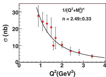
FIG. 16. (Color online) Fit to the cross section as a function of Q^2 distribution to determine scaling using data from the present experiment and CLAS data from Ref. [22].
