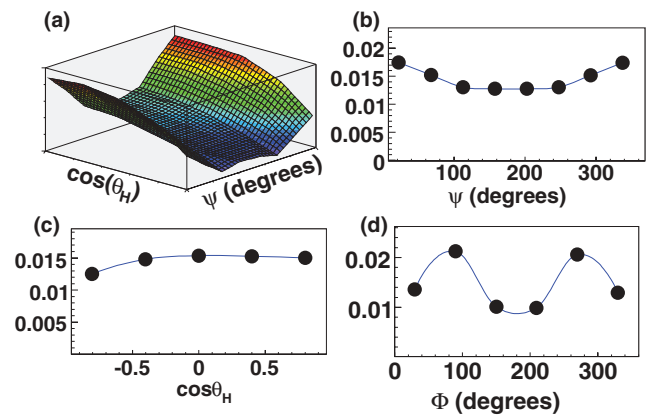
FIG. 9. (Color online) 2-D acceptance in \cos\theta_H and \psi , as well as the 1-D acceptance in \cos\theta_H , \psi , and \Phi . Error bars are not shown; the lines are present to guide the eye. The axes in the 2-D plot in (a) have the same range as that of the axis of the two 1-D plots in (b) and (c).
