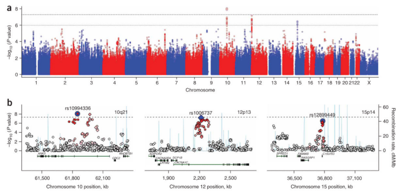
Figure 1. Association results for the combined analysis of the WTCCC, STEP-UCL and ED-DUB-STEP2 studies. (a) Genome-wide results ( -\log_{10}P ) are shown in chromosomal order for directly genotyped ( N= 325,690 ) and imputed ( N= 1,444,258 ) SNPs that were tested for association in the overall sample of 4,387 bipolar cases and 6,209 controls. Horizontal lines indicate a P value of 5 \times 10^{-8} (dashed) and 1 \times 10^{-6} (dotted). (b) Plots for the three regions of strongest association. Results ( -\log_{10}P ) are shown for directly genotyped (diamonds) and imputed (circles) SNPs. The most associated SNP for each region is shown in blue, and the color of the remaining markers reflects the linkage disequilibrium ( r^2 ) with the top SNP in each panel (increasing red hue associated with increasing r^2 ). The recombination rate (second y axis) is plotted in light blue and is based on the CEU HapMap population. The dashed horizontal line indicates a P= 5 \times 10^{-8} . Exons for each gene are represented by vertical bars, based on all isoforms available from the Mar 2006 UCSC genome browser assembly.
