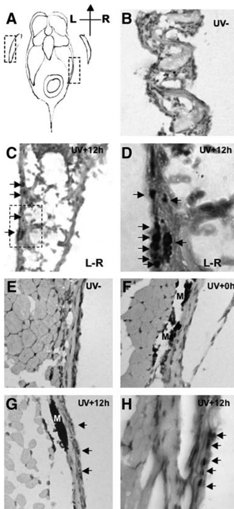
FIG. 4. Observation of DNA damage sites in zebrafish fin (B–D) and skin (E–H). Histological sections of adult zebrafish 12 hours after of UVB (2.16 kJ/m 2 ) exposure, stained with an antibody to detect phospho-histone H2AX (phospho-H2AX). (A) Schematic diagram of zebrafish section; dotted boxes denote the examined fin and skin tissues in (B) and (E), respectively. (B) Section of pectoral fin of untreated wt fish (hematoxylin and eosin stain; magnification 200×). (C) Section of pectoral fin of UVB exposed wt fish. Phospho-H2AX signals are located in the epidermis on the most outer side of fin (arrows); magnification 200×. Dotted box indicates region examined in (D). (D) High magnification (630×) view of the phospho-H2AX positive cells in the fin. (E) No phospho-H2AX signal is detected in the skin of untreated fish; magnification 200×. (F) Skin of fish sacrificed immediately after UVB exposure reveals no staining for phospho-H2AX; magnification 200×. (G) Skin at 12 hours postirradiation reveals specific phospho-H2AX staining; magnification 200×. (H) High magnification (630×) view of the phospho-H2AX positive cells in the skin. Phospho-H2AX positive nuclei are indicated with arrows; M denotes melanin.
