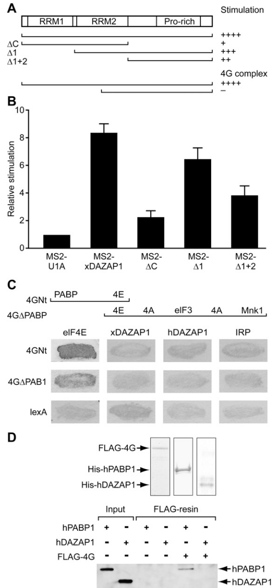
FIGURE 9. DAZAP1 C-terminal regions stimulate translation independently of a direct interaction with eIF4G. (A) Cartoon showing the constructs utilized in B, summarizing their relative ability to stimulate translation, and the co-isolation of eIF4G with full-length but not truncated GST-DAZAP1 in Yang et al. (2009). (B) Oocytes expressing MS2-U1A, MS2-xDAZAP1, MS2-ΔC (amino acids 1–192), MS2-Δ1 (amino acids 106–360), or MS2-Δ1+2 (amino acids 193–360) were co-injected with the luc-MS2 reporter and β-galactosidase control mRNAs. Data are plotted as in Figure 1A. (C, top) Cartoon showing the eIF4G truncations used and the relative locations of binding sites for the indicated partner proteins. (Bottom) Yeast two-hybrid assay using 4Gnt or 4GΔPABP or MS2 (negative control; indicated by lexA) fused to the LexA-DNA-binding domain and xDAZAP1, hDAZAP1, eIF4E (positive control), or IRP (iron-responsive protein, negative control) fused to the GAL4-activation domain. Interactions were detected by qualitative β-galactosidase filter assays. (D, top) SDS-PAGE analysis of the indicated purified recombinant proteins visualized with Gelcode Blue. (Bottom) Pull-down of Flag-tagged eIF4G (FLAG-4G) in the presence of purified His-tagged PABP1 or DAZAP1 analyzed by Western blot using anti-His antibodies.
