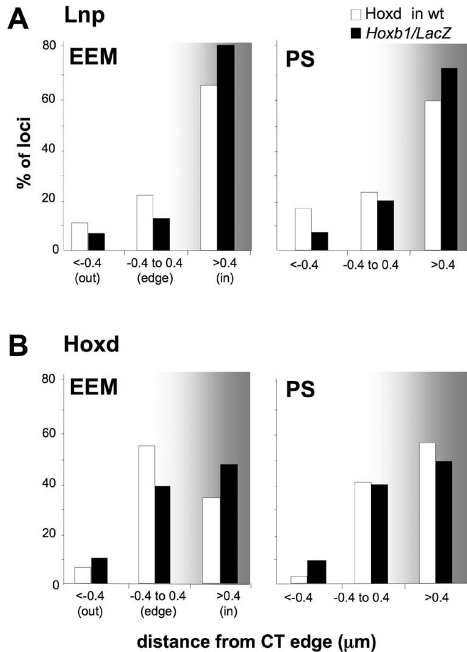
Figure 2. Hoxb1/LacZ nuclear reorganisation at E7.5 does not spread to flanking regions. Histograms showing the 3D positions of hybridisation signals for A) the Lnp and B) the Hoxd probe in nuclei from the EEM and the PS of wt (endog. Hoxd , white bars) or transgenic (black bars) E7.5 embryo.
