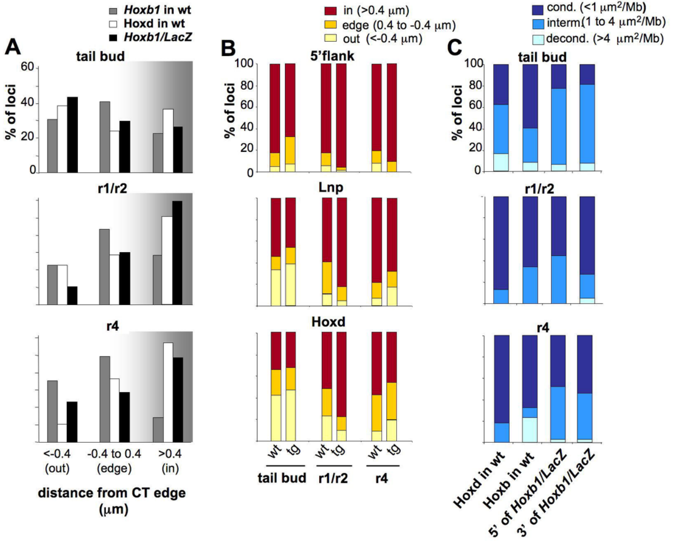
Figure 5. Nuclear reorganisation of the Hoxb1/LacZ transgene and surrounding regions along the antero-posterior axis of E9.5 embryos. (A) Histograms showing the percentage of Hoxb1/LacZ hybridisation signals inside, at the edge or outside of the MMU2 CT in the tailbud, r1/r2 or r4 or of E9.5 Hoxb1/LacZ embryos (black bars) compared to endogenous Hoxd (white bars) or endogenous Hoxb1 on MMU11 in wild-type E9.5 embryos (grey bars). (B) Histograms showing the percentage of signals located either inside (red bars), at the edge (orange bars) or outside (yellow bars) of the CT for the 5'flanking, the Lnp and the Hoxd probes in tailbud, r1/r2 or r4 of either wild-type (wt) or Hoxb1/LacZ transgenic (tg) embryos. (C) Percentages of nuclei showing condensed (dark blue), intermediate (blue) or decondensed (light blue) chromatin structures for the regions between Lnp and Hoxd probe signals ( Hoxd wt) and between Hoxb1 and Hoxb9 probe signals ( Hoxb wt) in tailbud, r1/r2 or r4 of wild-type embryos or between Lnp and Hoxb1/LacZ probe signals (5' Hoxb1/LacZ ) and between Hoxb1/LacZ and Hoxd probe signals (3' Hoxb1/LacZ ) in Hoxb1/LacZ embryos.
