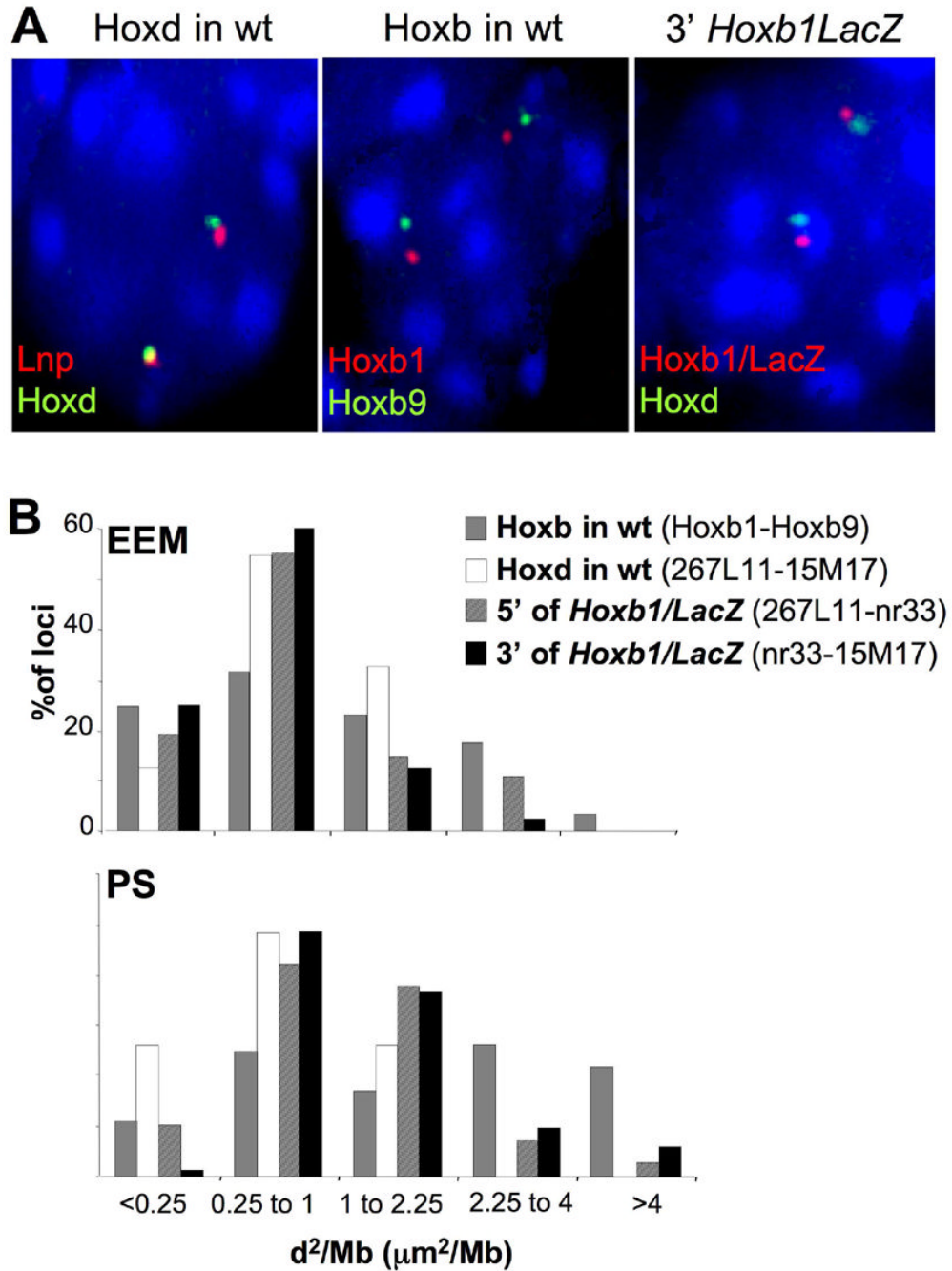
Figure 3. Chromatin decondensation in E7.5 transgenic embryos. (A) 3D DNA-FISH of, left panel; Lnp and Hoxd, middle panel; Hoxb1 and Hoxb9 probes on nuclei from the PS of E7.5 wild-type embryos, and of, right panel; Hoxb1/LacZ and Hoxd probes on nuclei from the PS of an E7.5 Hoxb1/LacZ embryo. Nuclei were counterstained with DAPI. Images are maximal projections of 3D stacks after deconvolution. (B) Distributions of mean-squared interphase distances ( d^2 ) in \mu m^2 normalised to genomic separation (in Mb) measured; between the Hoxb1 and Hoxb9 probes (grey bars) at endogenous Hoxb and between Lnp and Hoxd probes (white bars) at endogenous Hoxd in EEM and PS nuclei from E7.5 wt embryos, or
