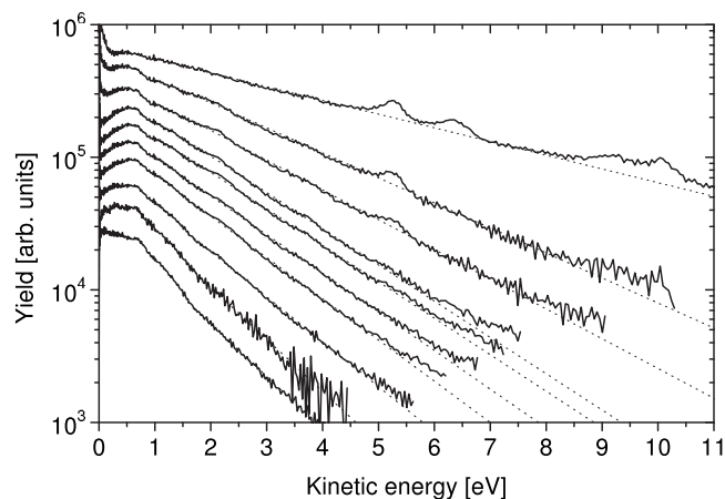
FIG. 2. Electron spectra of coronene at constant pulse duration of 150 fs. Wavelength of 775 nm. From bottom to top the laser intensities are as follows: 3.6, 4.9, 6.7, 8.0, 9.3, 10.9, 12, 21, 28, and 61 \times 10^{12} W/cm 2 . The spectra are shifted vertically for display purposes here and in all other photoelectron spectra.
