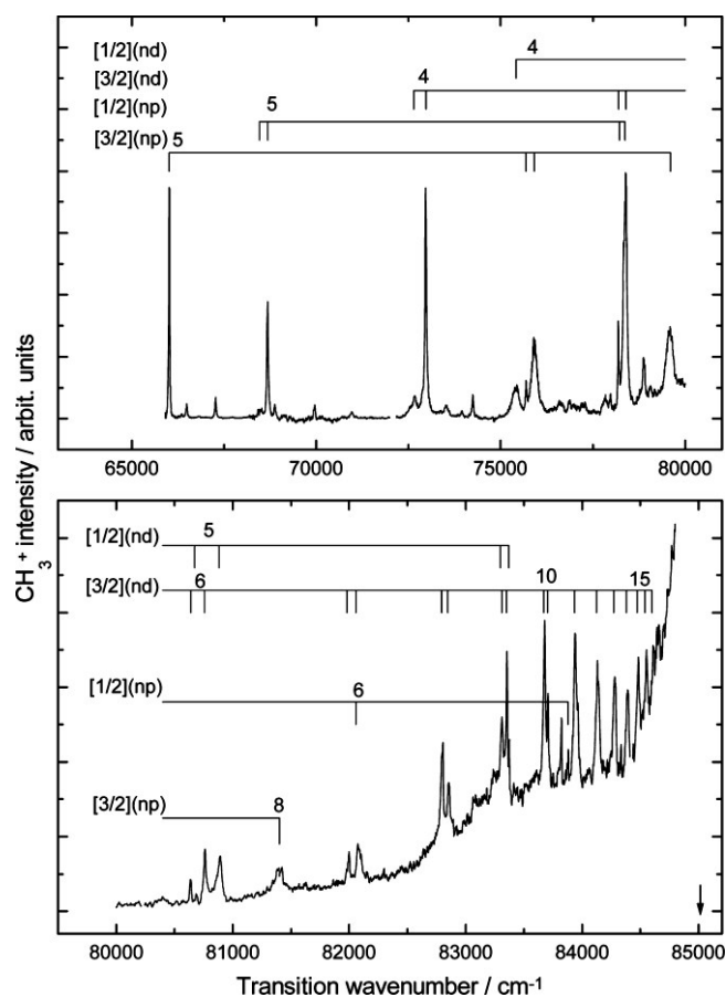
Figure 2. The power normalized (2 + 1) REMPI spectrum of jet-cooled \text{CH}_3\text{Br} between 65000 and 85000 \text{cm}^{-1} recorded with linearly polarized light. The first IE at 85031 \text{cm}^{-1} is indicated by an arrow.
