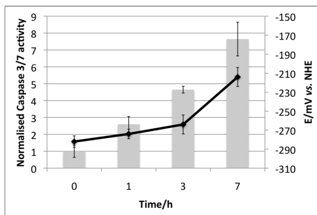
Figure 6. Intracellular potential measurements and caspase activity from mouse fibroblast cells undergoing hydrogen peroxide induced apoptosis. Diamonds represent potential measurements and columns represent measurements of caspase 3/7 activity. Error bars in potential measurements represent the standard deviation across ten single-cell measurements and error bars in caspase activity represent standard deviation across ten replicate wells.
