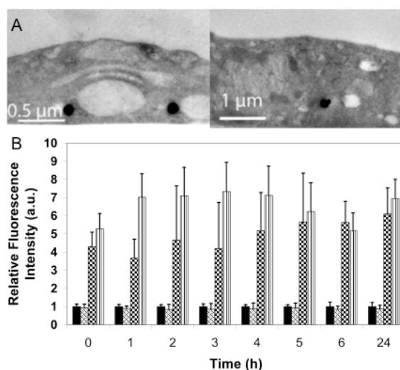
Figure 3. A) TEMs of nanosensors in 3T3 fibroblast cell B) Oxidative stress measured over 24 hours using DCFH-DA assay: Untreated cells (solid bar) Cells incubated with nanosensors (diagonally striped bar) Zn +ve control (chequered bar) t-BOOH +ve control (vertically striped bar).
