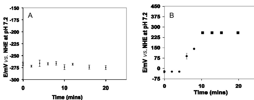
Figure 4. A) NQ-NS as a sensor for normoxic cellular potential measurements. B) HQ-NS as a sensor of oxidative stress caused by AAPH. Solid squares indicate potentials where HQ-NS is fully oxidised. Error bars indicate the standard deviation of potentials calculated from spectra recorded during three independent experiments.
