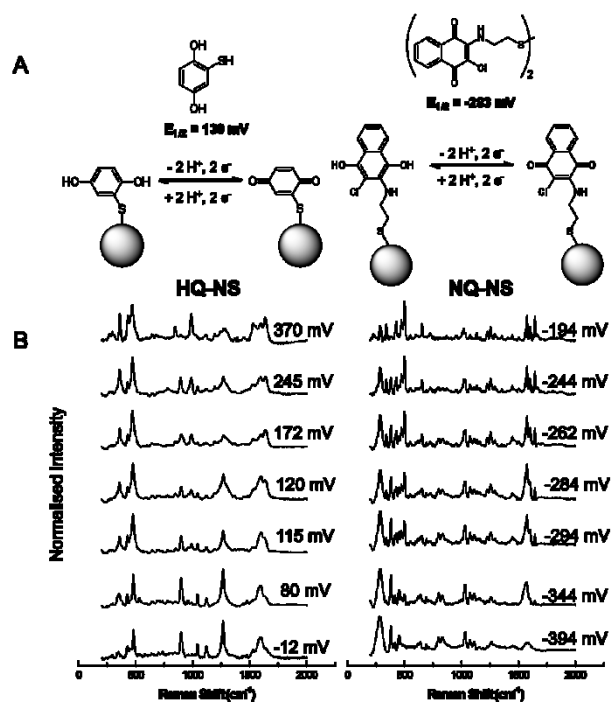
Figure 1. SERS Nanosensors. A – structures, electron transfer schemes and standard reduction potentials; B – potential dependent changes in SERS spectra.
