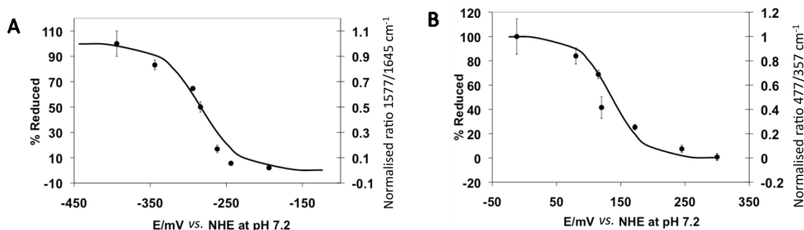
Figure 2. Redox potential ranges covered by SERS nanosensors. A) NQ-NS and B) HQ-NS . Error bars show the standard deviation of three independent measurements. Points indicate SERS spectroscopic measurements and solid lines represent plots of the Nernst Equation on the basis of half-wave potentials measured using cyclic voltammetry.
