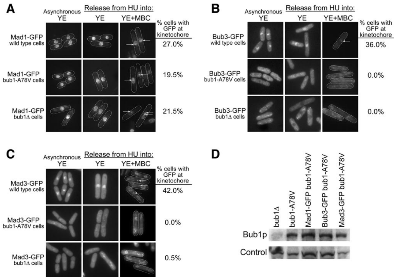
Figure 5. Bub3-GFP and Mad3-GFP do not localize to kinetochores when the SAC is activated in bub1-A78V cells. Asynchronous wild-type, bub1-A78V , and bub1Δ cells expressing C terminally GFP-tagged Mad1 , Bub3 , or Mad3 driven by their native promoters at their endogenous loci were cultured in rich YE medium (Asynchronous YE) or synchronized in S phase by hydroxyurea (HU) to enrich for mitotic cells upon release into YE (YE) or into YE with MBC (YE+MBC), which activates the SAC. GFP localization was observed in live cells. Arrows denote kinetochore localization of the GFP-tagged protein. The percentage of cells exhibiting kinetochore localization of the GFP fusion protein was determined 2 h after release into YE+MBC. (A) Wild-type, bub1-A78V and bub1Δ cells expressing Mad1-GFP. (B) Wild-type, bub1-A78V , and bub1Δ cells expressing Bub3-GFP. (C) Wild-type, bub1-A78V , and bub1Δ cells expressing Mad3-GFP. (D) Western blot using an anti-Bub1p polyclonal antibody to determine levels of Bub1p-A78V in the strains examined in A–C.
