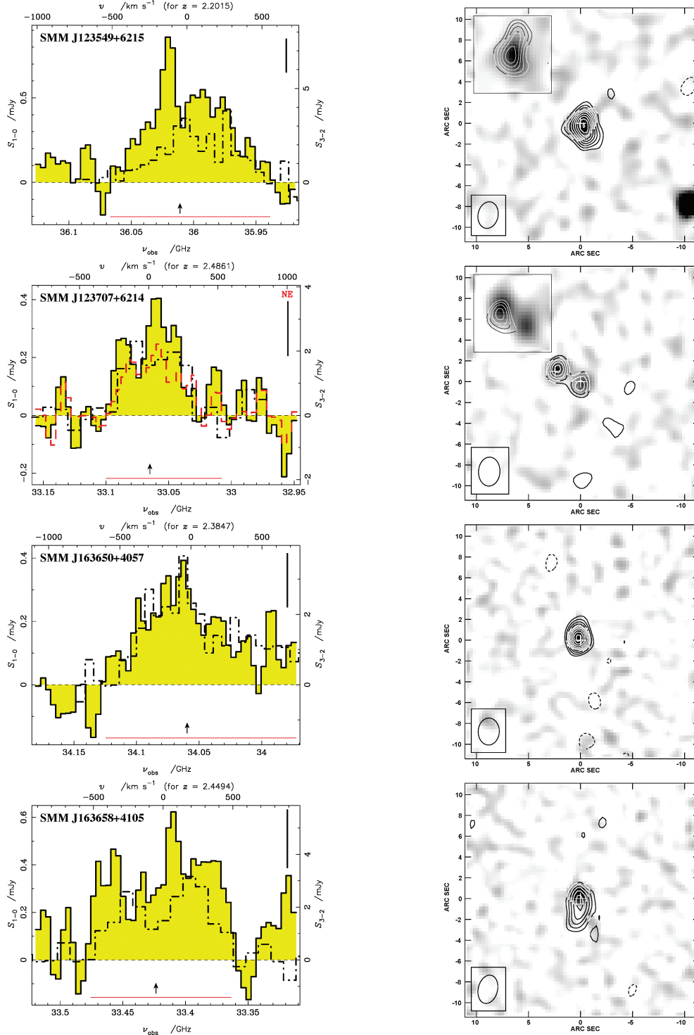
Figure 1. CO J=1-0 spectra and lightly CLEANED images for the SMGs in our study. On the left we show the spectra, integrated over a region of \sim 3 beam areas in the data cubes, with the corresponding PdBI CO J=3-2 spectra from Tacconi et al. (2006) shown as dot-dashed lines, scaled by 9^{-1} times to be on the same Rayleigh–Jeans T_b scale. Arrows indicate the CO J=3-2 line centres. The CO J=1-0 spectrum of the NE component of SMM J123707 is shown in red. All our targets are well detected with CO J=1-0 FWHM of \sim 300 – 800 km s^{-1} , marginally broader than the corresponding CO J=3-2 emission. The frequency range used to create the images in the right-hand panels are indicated below each spectrum. A typical \pm 1\sigma error bar is shown at the top right of each panel. Velocities are relative to the CO J=1-0 redshifts listed in Table 2 and the spectra have been Hanning smoothed with an four-channel triangular kernel with 4-MHz ( \sim 35 km s^{-1} ) spectral resolution. Right: CO J=1-0 emission integrated over the channels indicated in the corresponding spectrum, displayed as contours ( -3, 3, 4, \dots \times \sigma where \sigma is typically \sim 20 \mu Jy beam ^{-1} ), superimposed on linear grey-scales of the 1.4-GHz continuum emission. We see that all targets are marginally or well resolved at the resolution of our map, with SMM J123707 comprising two components. The beam is shown in the bottom left corner of each image. Insets show 6 \times 6 arcsec ^2 postage stamps of CO J=1-0 for SMM J123549 (a 220-km s^{-1} wide bin centred at -150 km s^{-1} , displayed as contours, superimposed on a grey-scale of the total CO J=1-0 emission) and SMM J123707 (contiguous 390-km s^{-1} wide blue and red bins represented by the contours and the underlying grey-scale, respectively, illustrating the velocity gradient across SMM J123707-NE).
