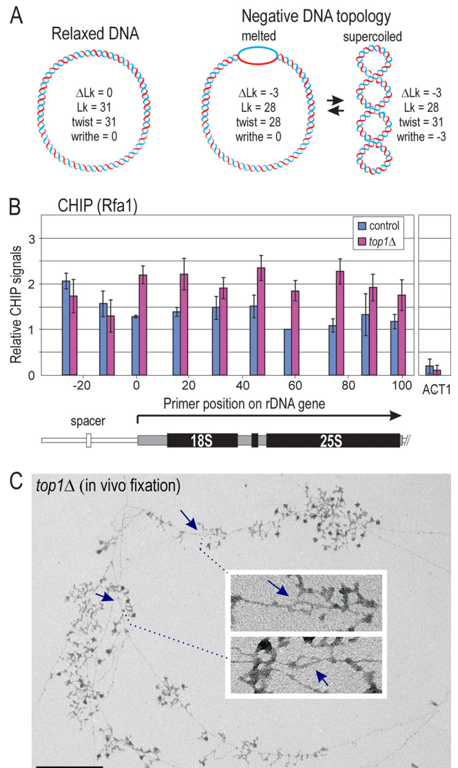
FIG. 6. Evidence that some negative topological stress occurs as melted DNA in top1Δ cells in vivo . (A) Schematic of the two inter-convertible forms of DNA under negative topological stress: melted versus negatively supercoiled. Shown is a hypothetical DNA plasmid of 325 bp, which has a relaxed linking number ( Lk_0 ) of 31 (i.e., 325/10.5 = 31 ). The linking number (Lk) has contributions from twist and writhe, i.e., Lk = \text{twist} + \text{writhe} . Relaxed plasmid on left has linking number (Lk) of 31 due to 31 helical twists, and thus its \Delta Lk = 0 , where \Delta Lk = Lk - Lk_0 (difference between the actual and the relaxed linking number). On the right is a plasmid of the same length but under negative topological stress ( \Delta Lk = -3 ), which can be relieved by melting a portion of the DNA or by negative writhe, both of which allow maintenance of stable B-form helix in most of the DNA. (B) ChIP analysis of occupancy of single-stranded DNA-binding protein RPA large subunit (encoded by RFA1 ) over the rDNA repeat and on ACT1 gene. Shown are the relative ChIP signals in control strain YB169 ( TAP-RFA1 ) versus top1Δ strain YB168 ( top1Δ , TAP-RFA1 ) after normalization to the rDNA5 primer within the rRNA gene. Error bars show standard error of the mean for three independent experiments. (C) EM images of several rRNA genes using modified Miller spreading conditions in which formaldehyde is added to cells prior to cell disruption, mimicking conditions used for ChIP fixation. Arrows indicate topo-bubbles in two nearby genes. Bubbles shown enlarged in the inset. Bar, 0.5 \mu\text{m} .
