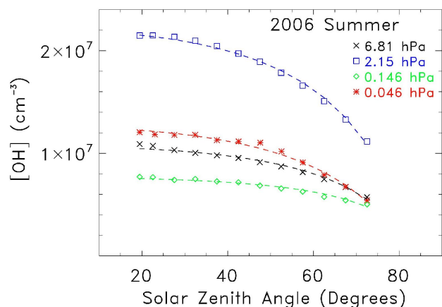
Fig. 3. Hydroxyl concentrations at 6.81 hPa (black x's), 2.15 hPa (blue squares), 0.146 hPa (green diamonds), and 0.046 hPa (red *) obtained from full-day (morning+afternoon) averages within 5° solar zenith angle bins. Corresponding dashed curves show exponential function fits as described in the text.
