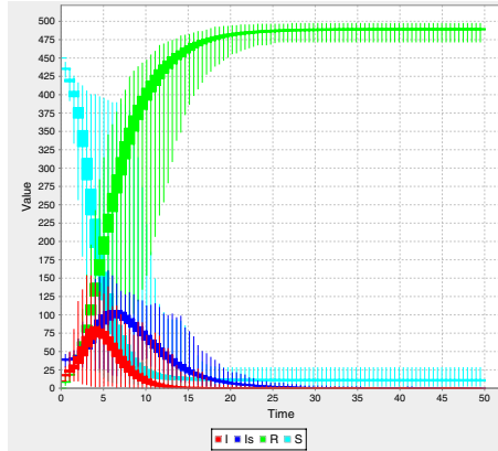
Fig. 9. Simulation results for the SII s R model with locations (island-type) and without drug treatment: confidence intervals, all species (Gillespie’s direct method, average of 100 runs). The thick lines (bars) represent the endpoint of the confidence intervals (with confidence level 1 - \alpha = 0.95 ) whereas the thin lines (shadows) illustrates the highest and the lowest values obtained from the set of simulation runs.
