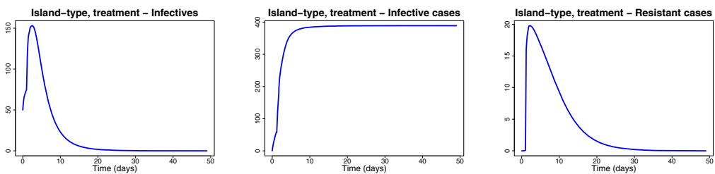
Fig. 15. Simulation results for the SII_sR model with treatment/prophylaxis, drug resistance and locations (island-type): instantaneous number of total infectives at a given time point (left), cumulative number of total infectives (middle) and total resistant cases (right).
