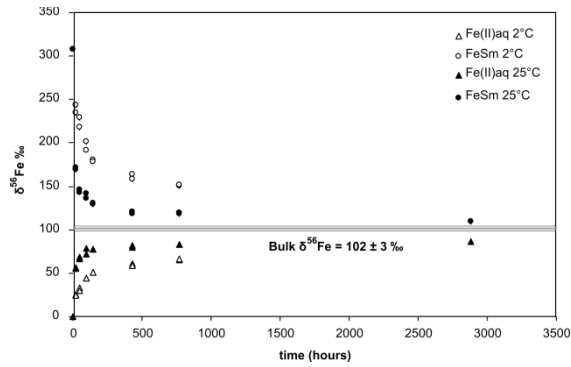
Fig. 3: Time evolution of Fe isotope compositions of \text{FeS}_m (circles) and \text{Fe(II)}_{\text{aq}} (triangles) at 25^\circ\text{C} (filled signs) and 2^\circ\text{C} (open signs). 2^\circ\text{C} experiments were stopped after one month. 25^\circ\text{C} experiments were stopped after four months. The grey area is the bulk composition of the system including errors.
