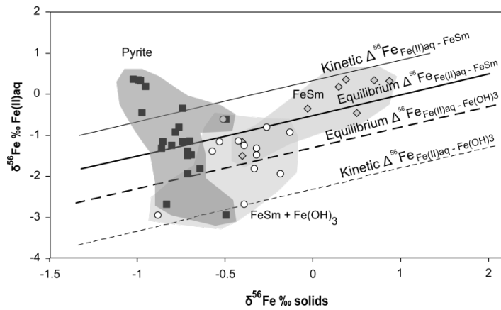
Fig. 7: Plot of the isotopic compositions of pore water versus the solid highly reactive iron phases, modified after Johnson et al. (2008). Data for pyrite (filled squares) and HCl extracted phases (grey diamonds and open circles) are from Severmann et al. (2006). Compositions for FeS m were derived from HCl extraction data where Fe(II) HCl > 80%, as suggested by Johnson et al. (2008). Kinetic \Delta^{56}\text{Fe}_{\text{Fe(II)aq-FeS}_m} are from Butler et al. (2005). We used our 2°C values for equilibrium \Delta^{56}\text{Fe}_{\text{Fe(II)aq-FeS}_m} . Kinetic and equilibrium \Delta^{56}\text{Fe}_{\text{Fe(II)aq-Fe(OH)}_3} are from Johnson et al. (2004).
