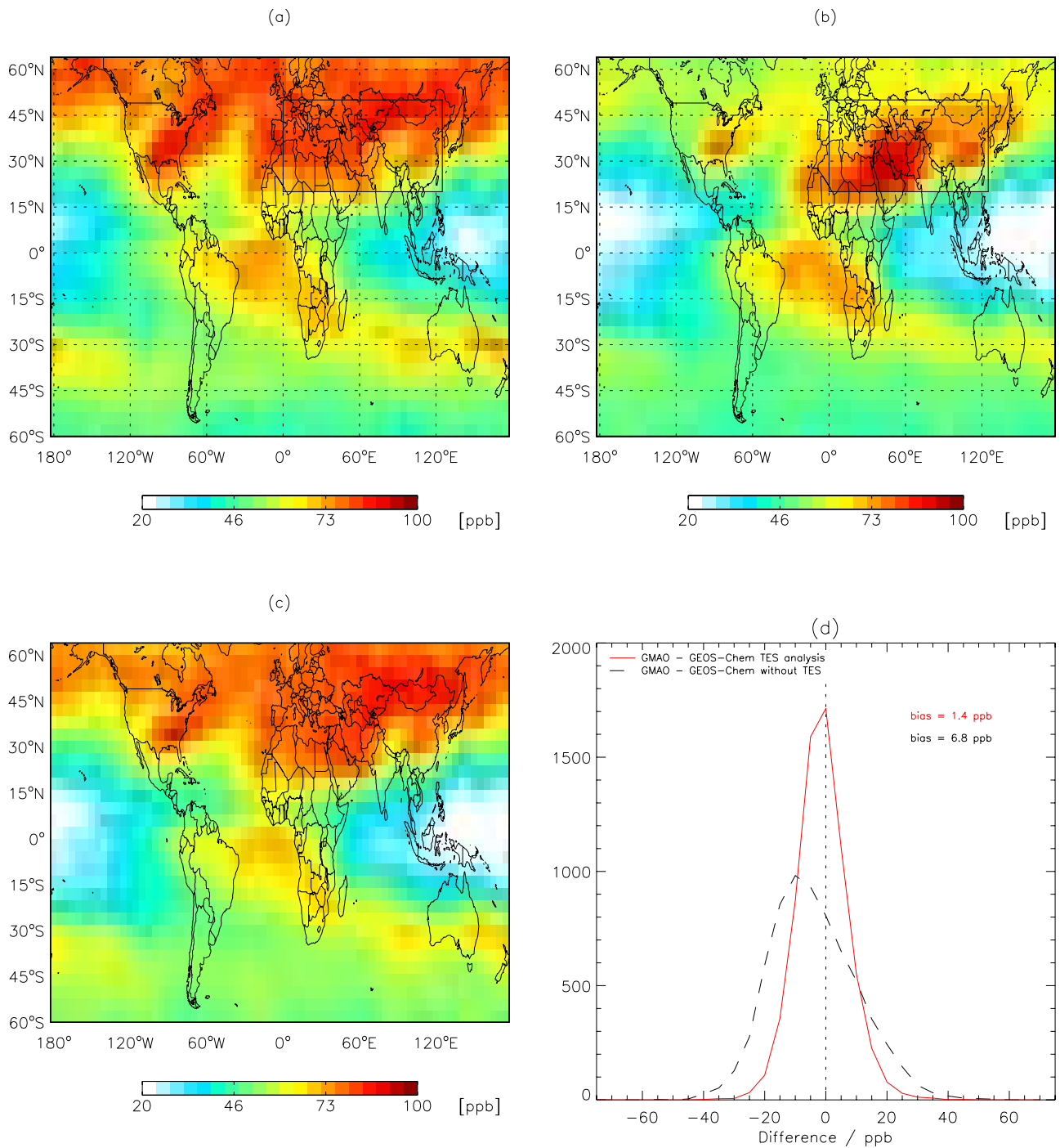
Figure 10. Mean August 2006 ozone distribution at 7–8 km produced by (a) assimilation of OMI and MLS data into the GMAO GEOS-4 GCM, (b) the GEOS-Chem model, and (c) the GEOS-Chem model after assimilation of bias-corrected TES data following Nassar et al. [2008]. (d) Histogram of the differences in ozone between the GMAO ozone assimilation and the GEOS-Chem model with (red line) and without (black dashed line) assimilation of TES data. The ozone differences were calculated over the region indicated by the box in Figures 10a and 10b and are based on daily modeled fields at 0 GMT.
