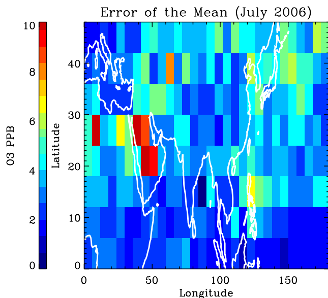
Figure 3a. Standard error of the mean for the July 2006 ozone values at 464 hPa.
