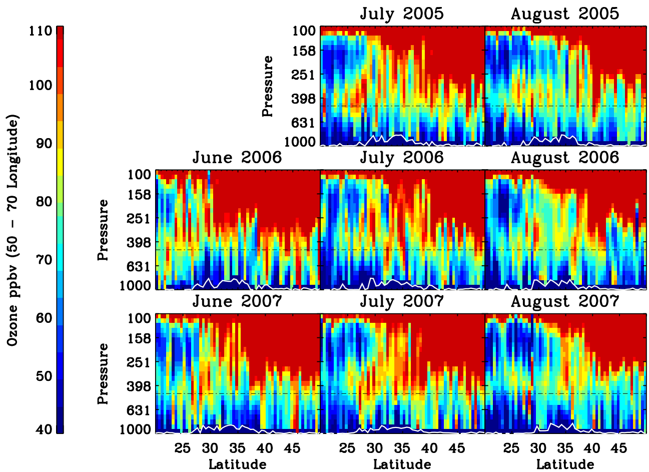
Figure 8. TES observed vertical ozone distributions for longitudes between 50° and 70°E. The white line indicates the average surface pressure. Data are not corrected for the approximately 15% TES bias.
