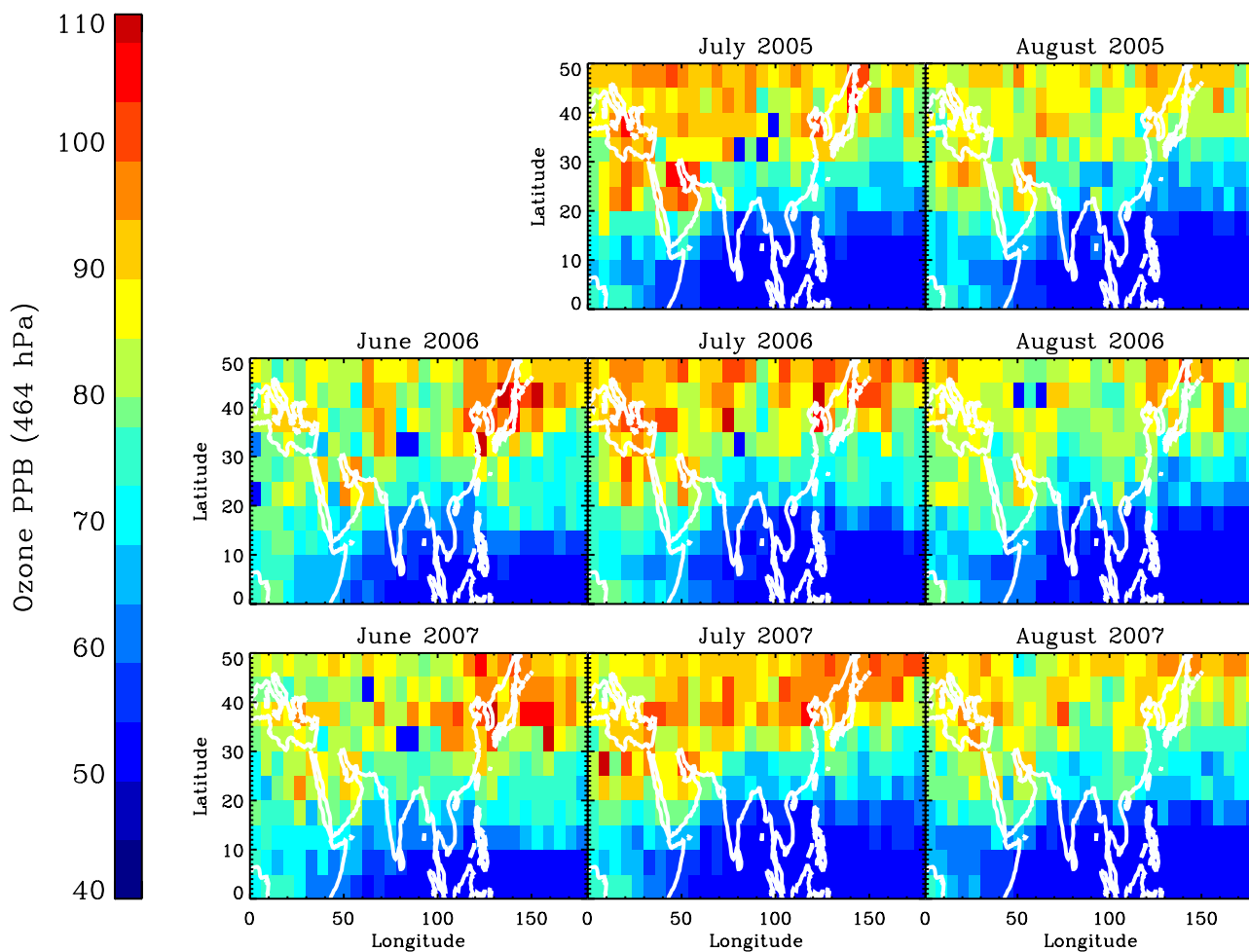
Figure 2. TES monthly averaged ozone at 464 hPa. Data are gridded onto 6^\circ \times 6^\circ bins. There are no data for June 2005 as TES was undergoing operational difficulties during that time period. Data are not corrected for the approximately 15% TES bias.
