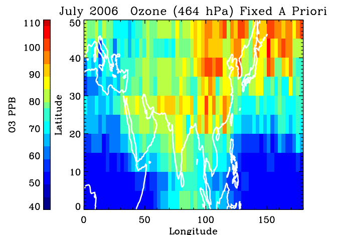
Figure 3c. TES estimate of ozone at 464 hPa if we use a fixed a priori constraint vector.
