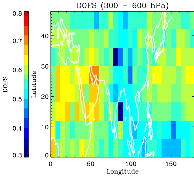
Figure 3b. DOFS for the region between 300 and 600 hPa.
