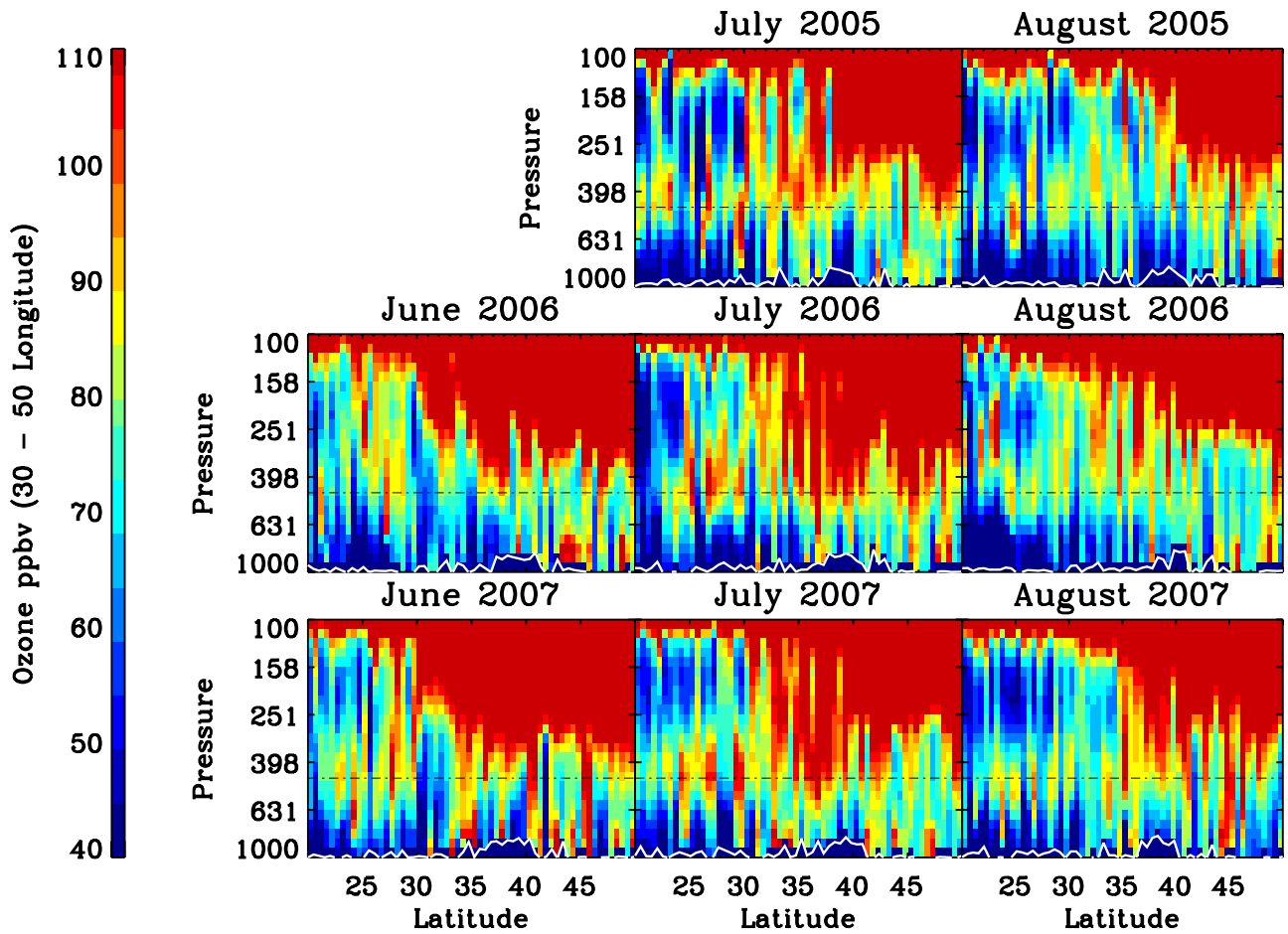
Figure 9. TES observed vertical ozone distributions for longitudes between 30° and 50°E. The white line indicates the average surface pressure. Data are not corrected for the approximately 15% TES bias.
