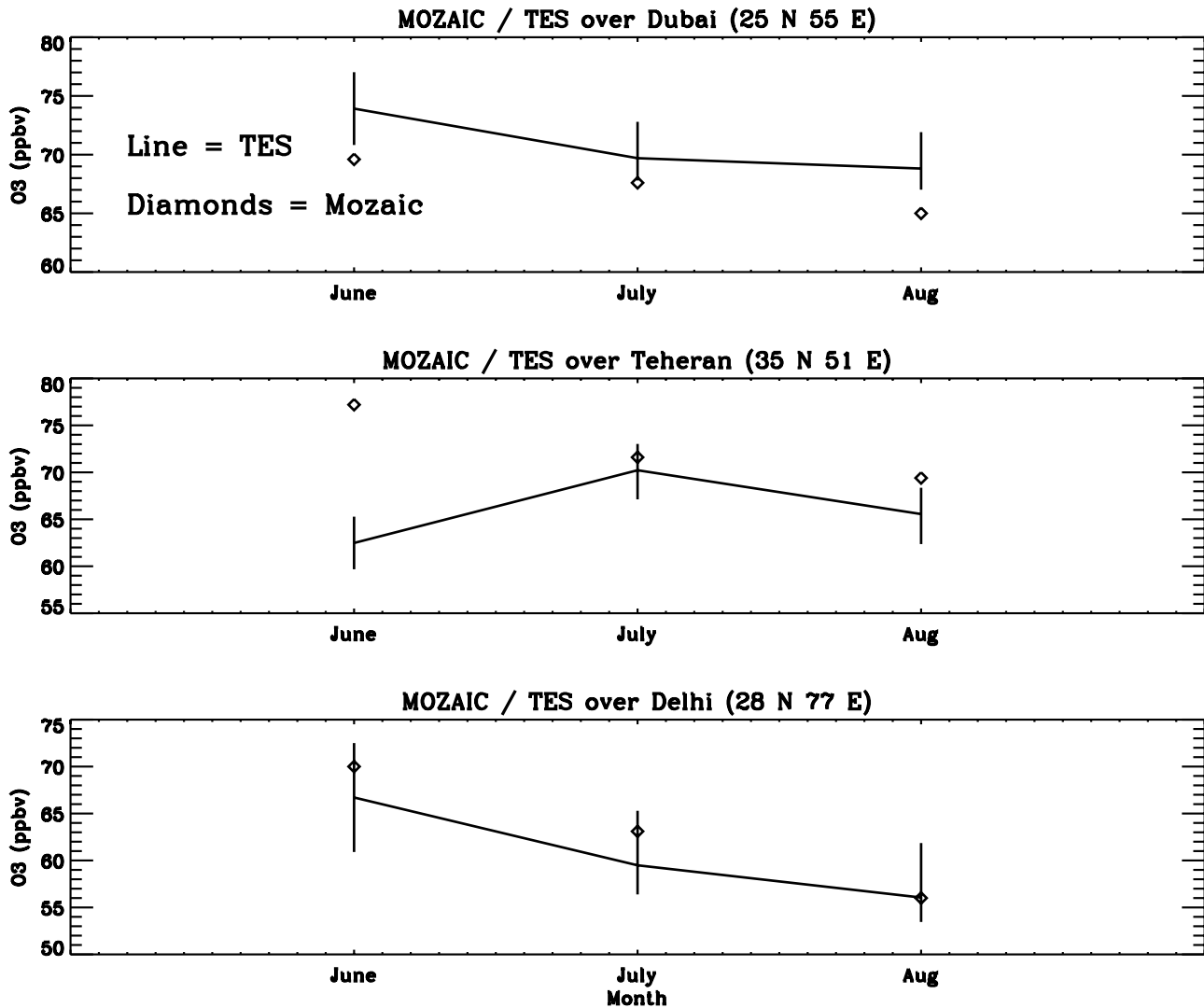
Figure 4. Comparison between 10-year climatologies derived from MOZAIC ozone measurements and a 3-year climatology derived from TES ozone observations. The error bars are the standard error on the mean for the TES ozone measurements. The TES ozone values have been decreased by 12% to account for the 10–15% TES bias.
