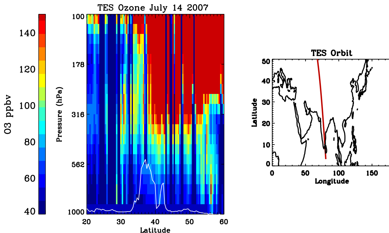
Figure 7. TES ozone profiles from the “step and stare” mode. There is approximately 1 observation every 35 km. The white line is the average surface pressure. Data are not corrected for the approximately 15% TES bias.
