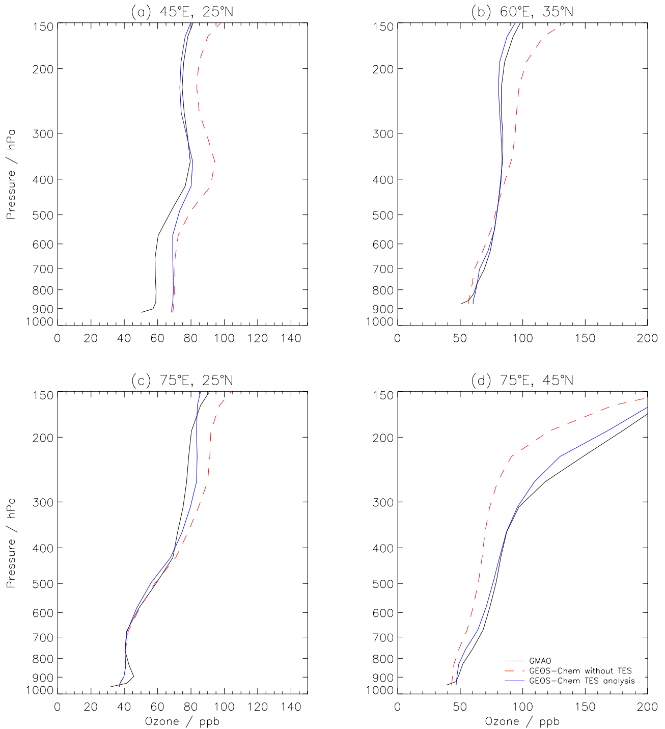
Figure 11. Comparison mean modeled profiles across the Middle East and Asia for August 2006. The black line shows the profiles from the assimilation of OMI and MLS ozone data into the GMAO GEOS-4 GCM, the blue line indicates the profiles from the assimilation of TES ozone data into the GEOS-Chem model, and the red dotted lines are the GEOS-Chem profiles obtained without assimilation of TES data.
