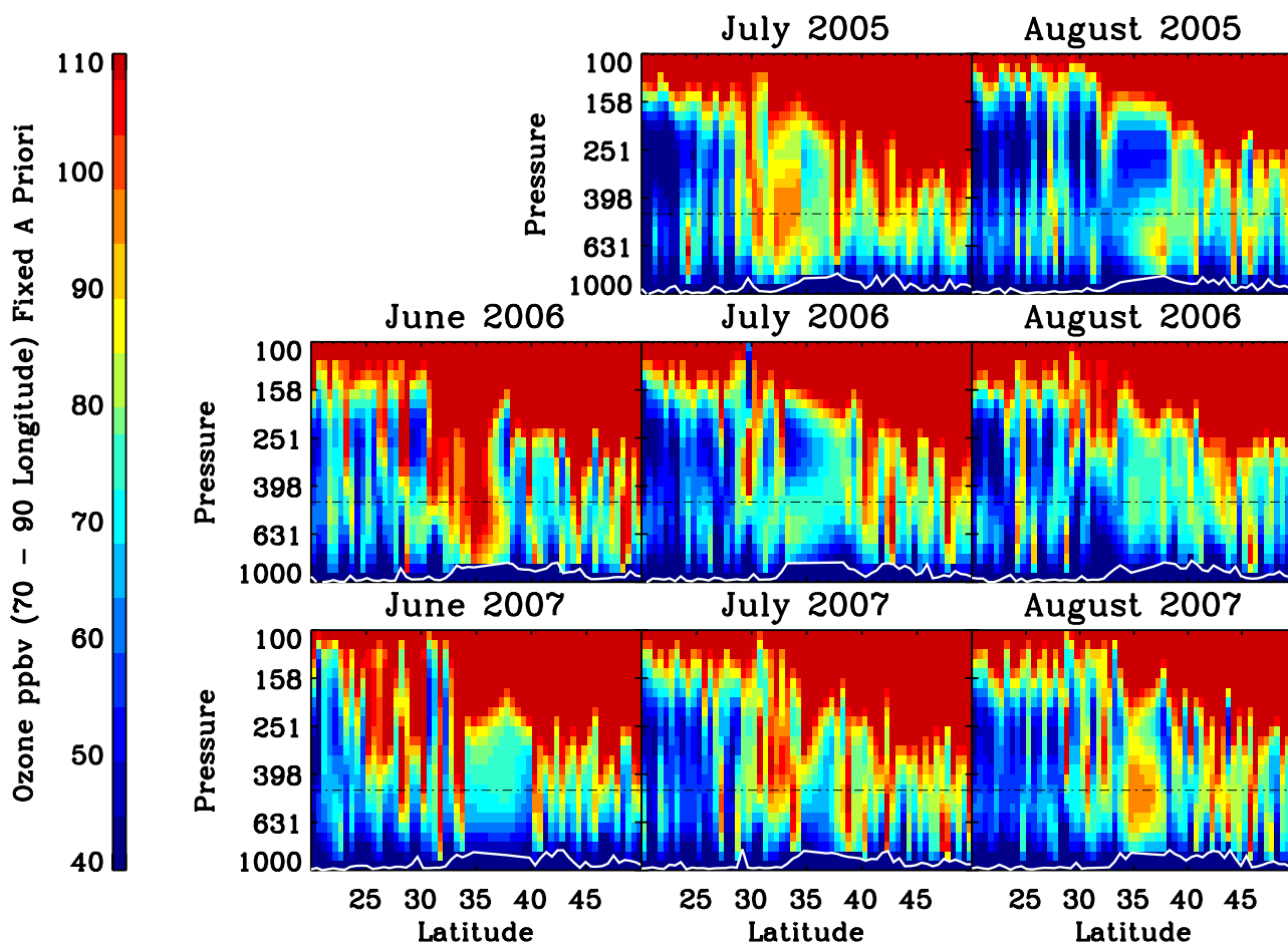
Figure 6. Same as in Figure 5 except the ozone profiles have been recalculated using a fixed a priori constraint.
