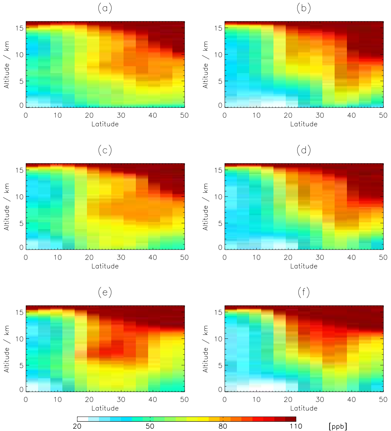
Figure 12. Monthly mean altitude-latitude cross sections of modeled ozone abundances for August 2006 along (left) 45°E and (right) 70°E for (a)–(b) the GEOS-4 GCM with assimilated observations from OMI and MLS, (c)–(d) the GEOS-Chem model with assimilated data from TES, and (e)–(f) the GEOS-Chem model without assimilation of TES data.
